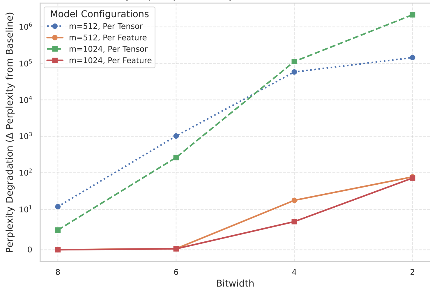
Dictionary Capacity Sensitivity: Robustness vs. Scale Tradeoff
