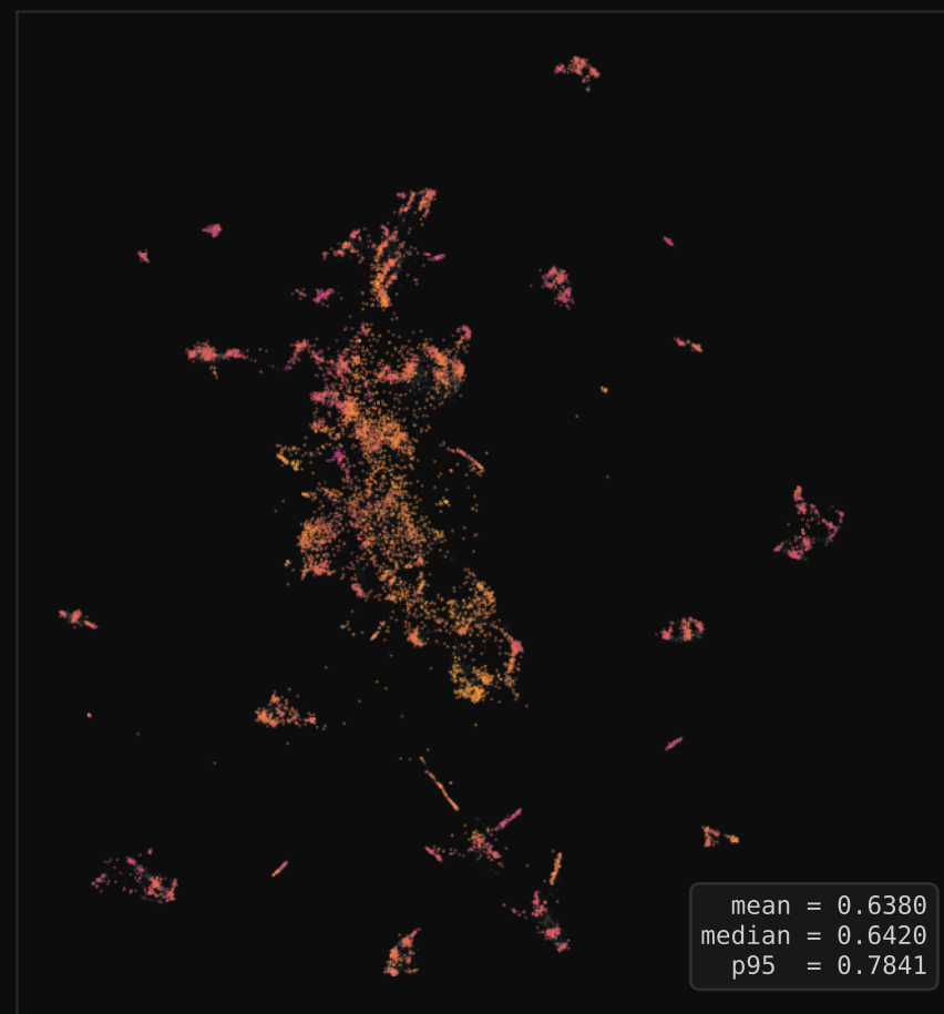
Per-Feature 6-bit
