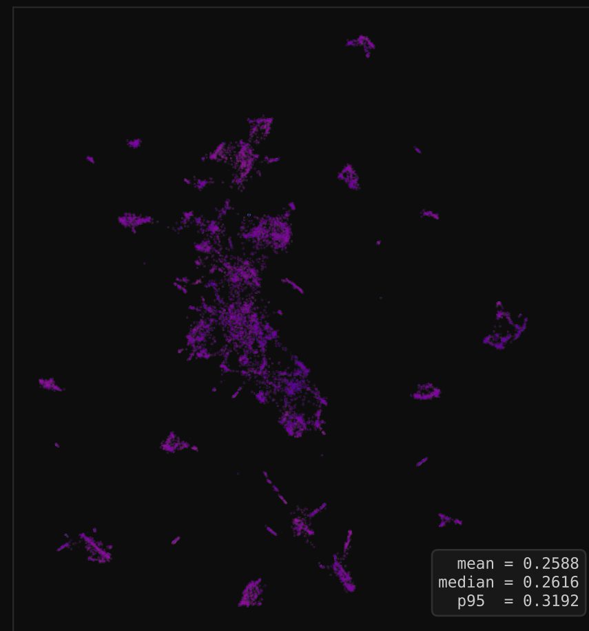
Per-Feature 8-bit
