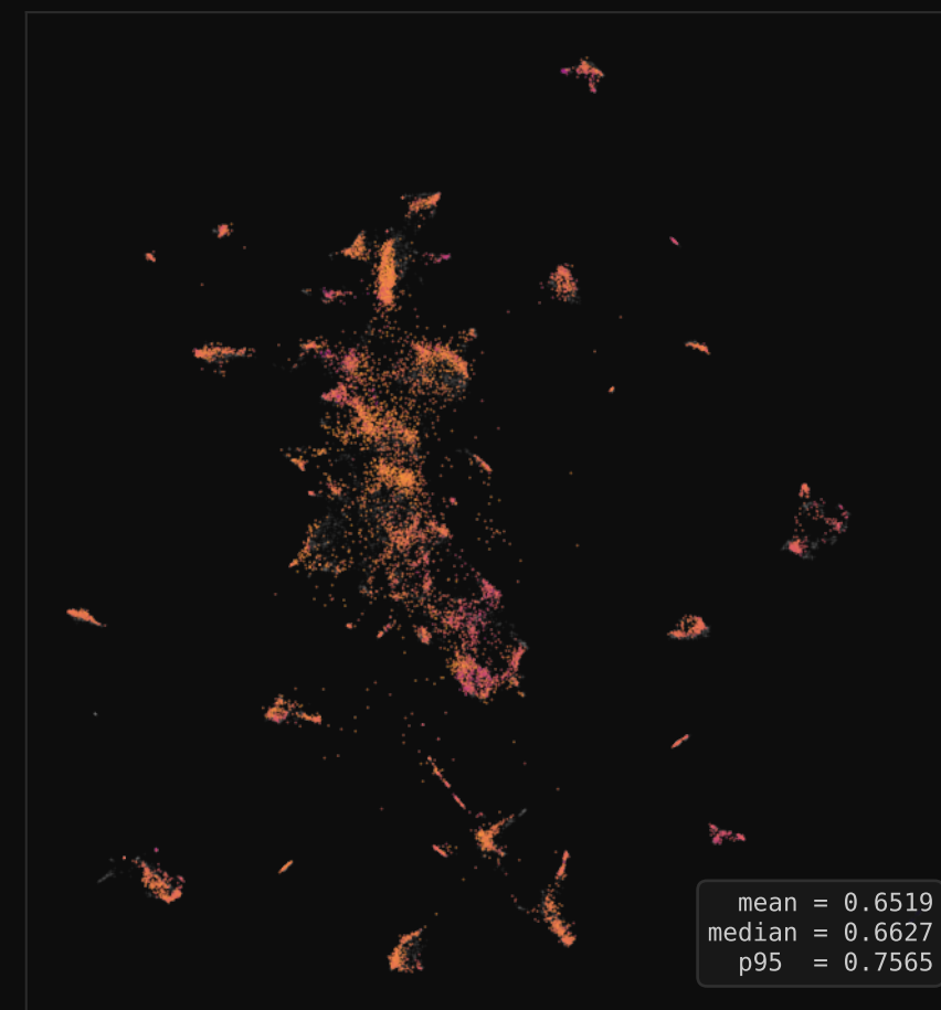
Per-Feature 2-bit
