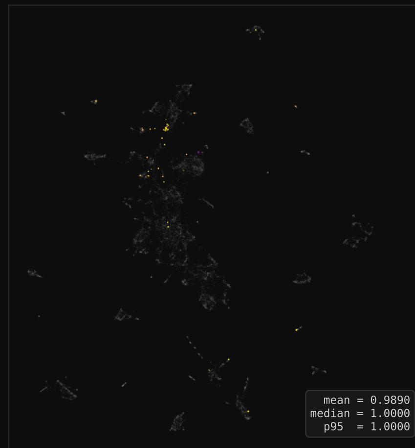
Per-Feature 4-bit
