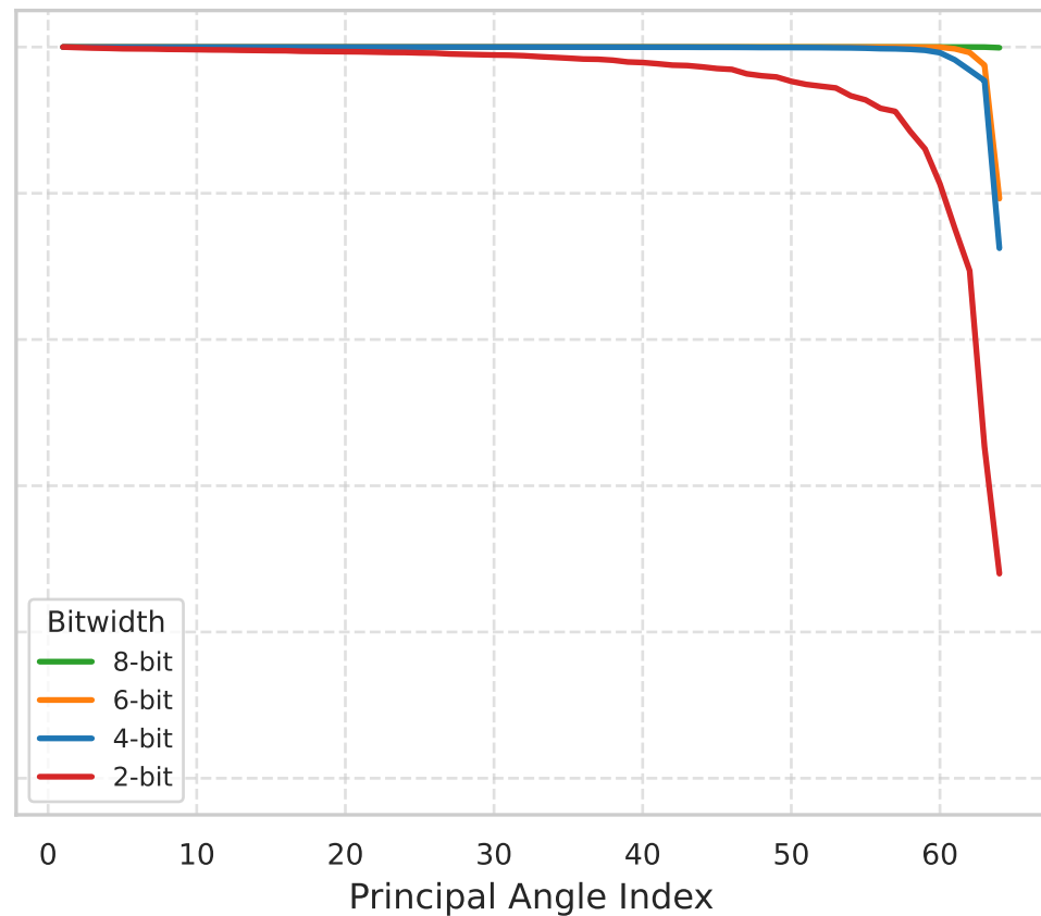
Per-Feature (k=64)
