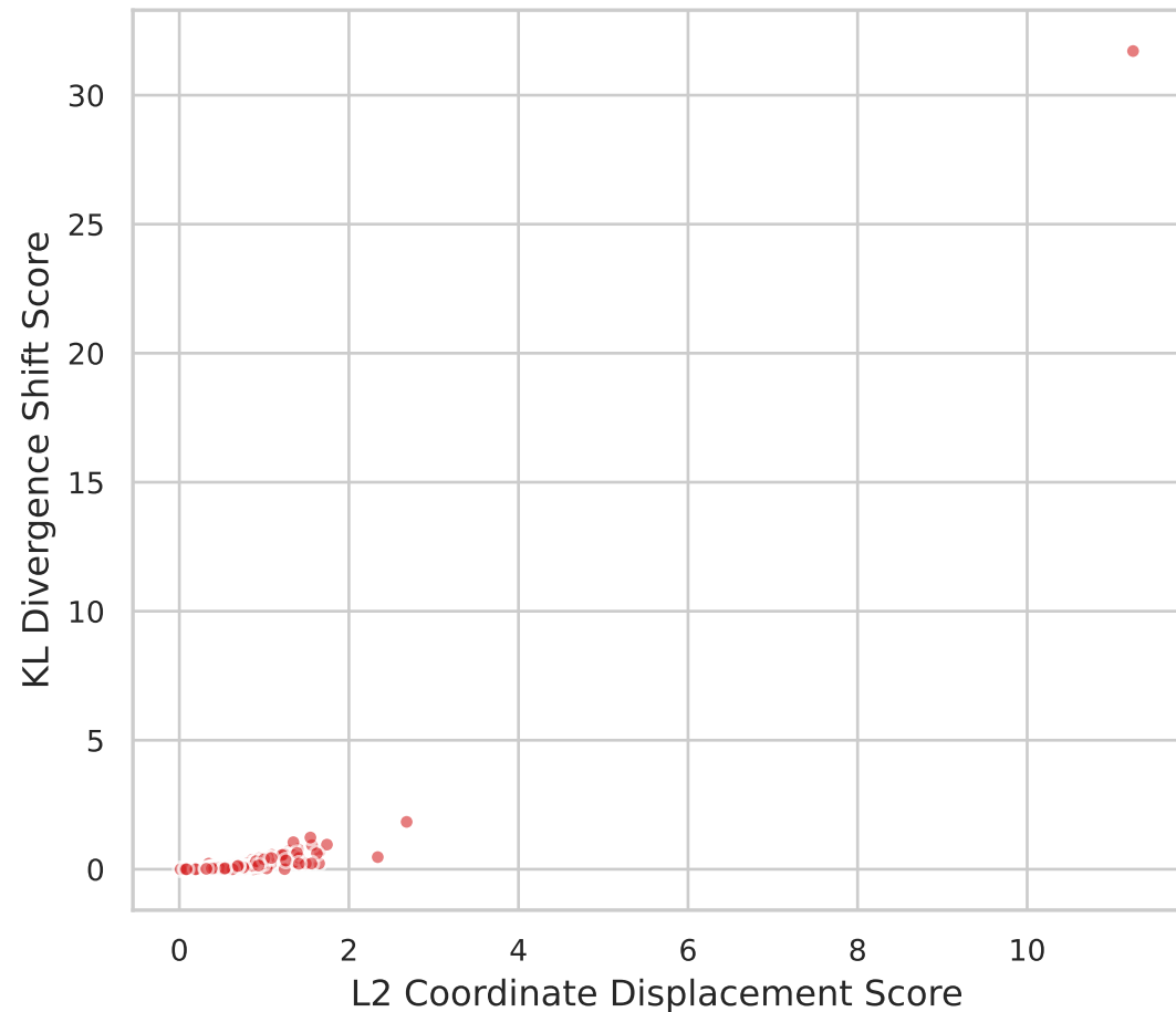
Per-Tensor (4-bit)
