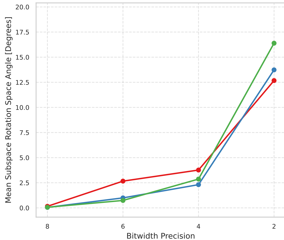
Bottleneck Capacity m = 512 (Per-Feature Strategy)
