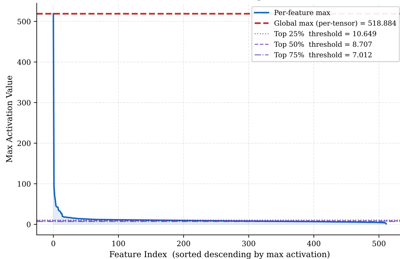
Per-Feature Activation Range, m = 512
