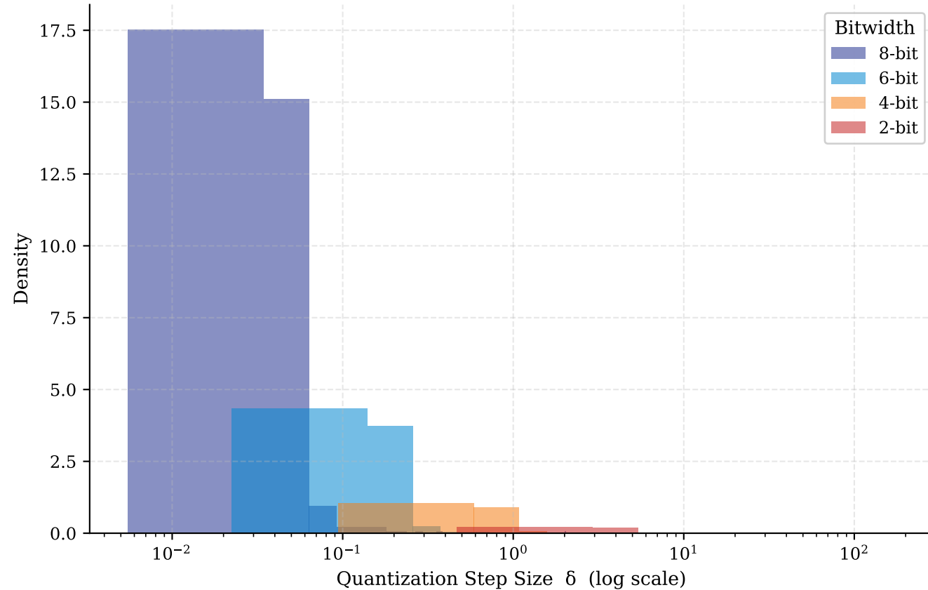
Per-Feature Step Size Distribution, m = 512
