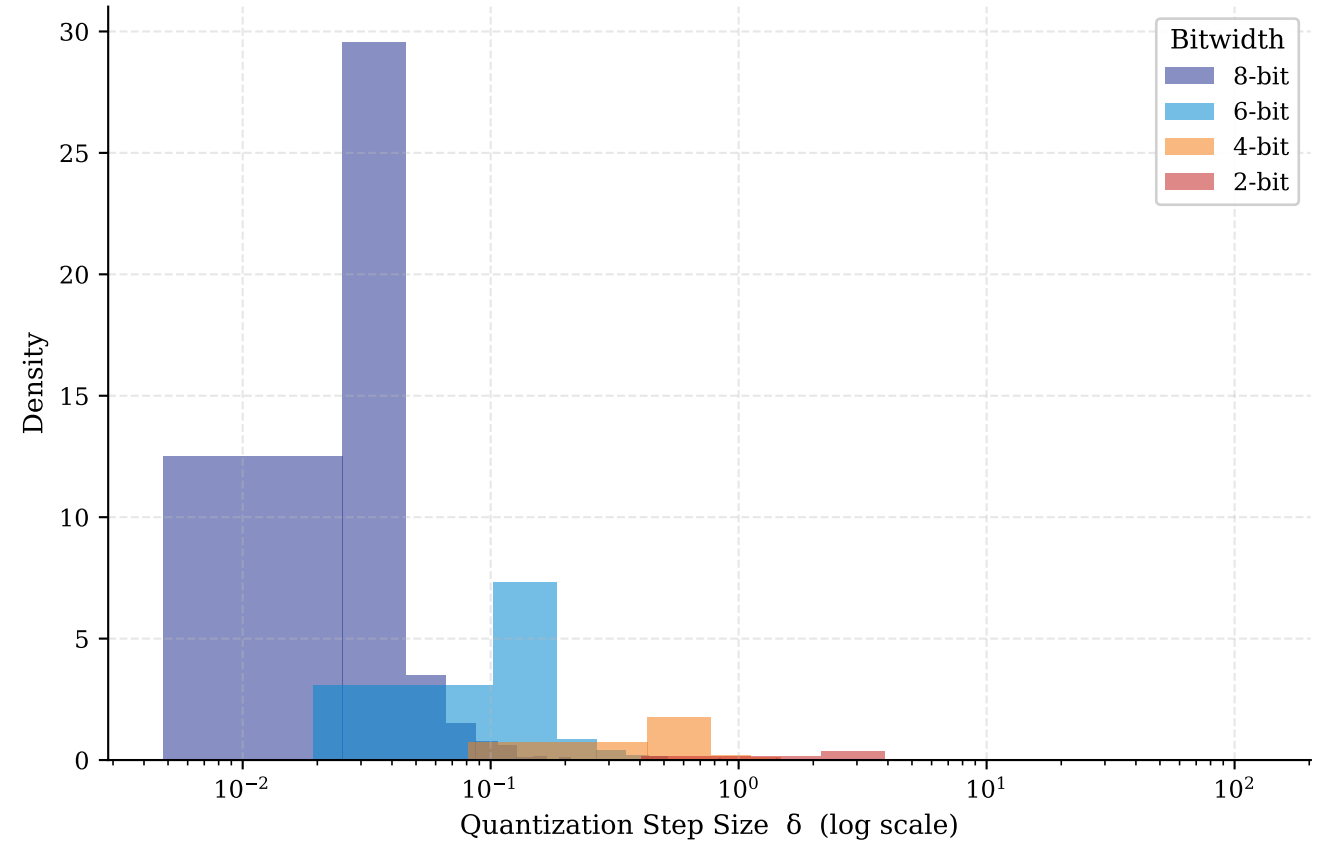
Per-Feature Step Size Distribution, m = 1024
