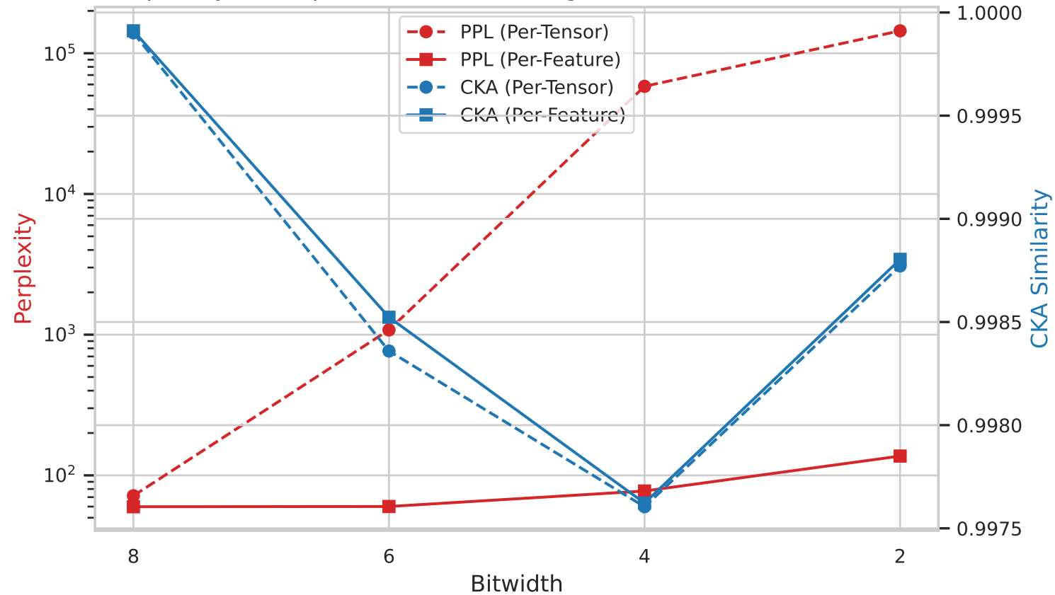
Perplexity vs. Representation CKA Alignment (Bottleneck m = 512 )
