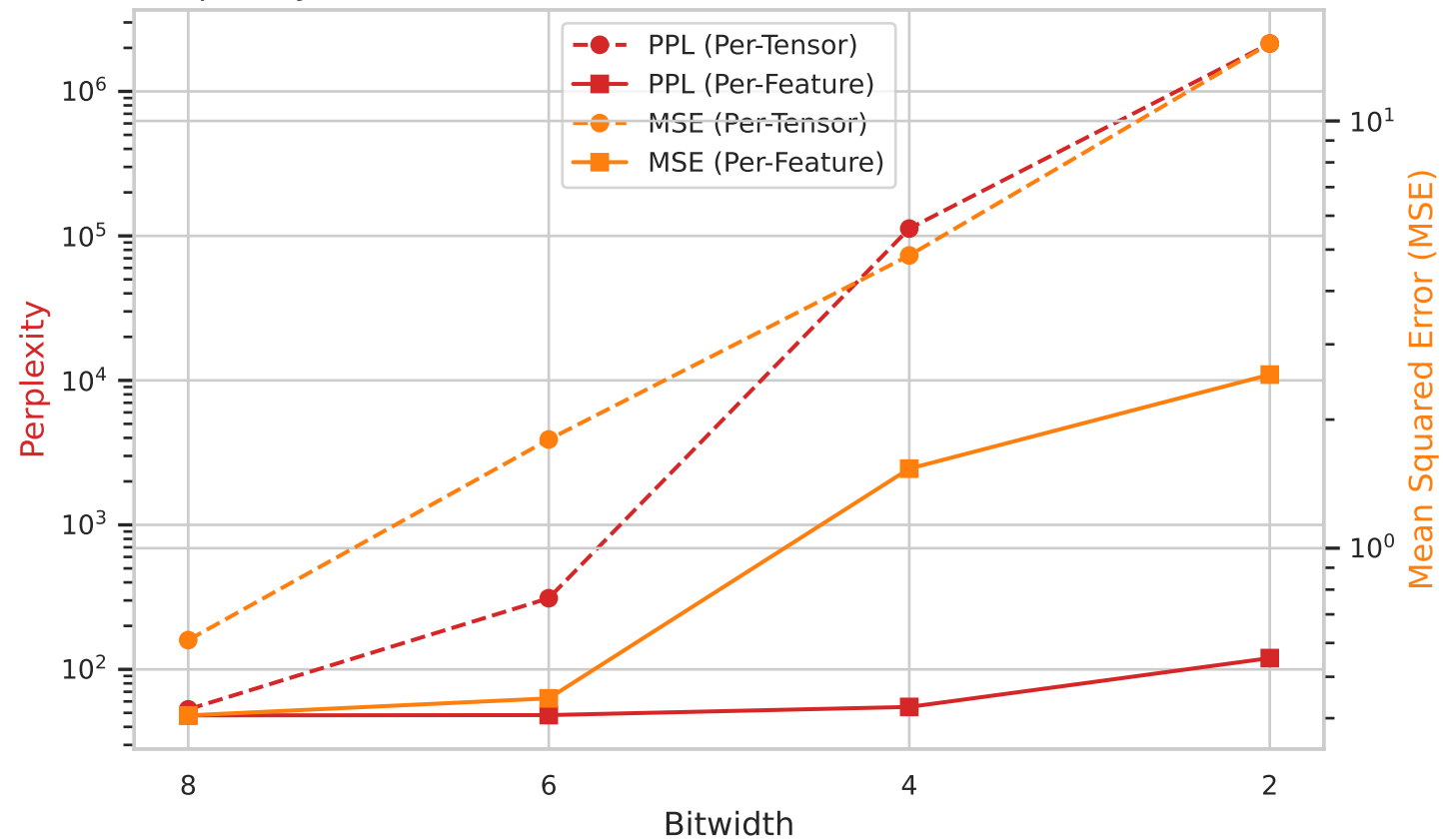
Perplexity vs. Activation Reconstruction MSE (Bottleneck m = 1024 )
