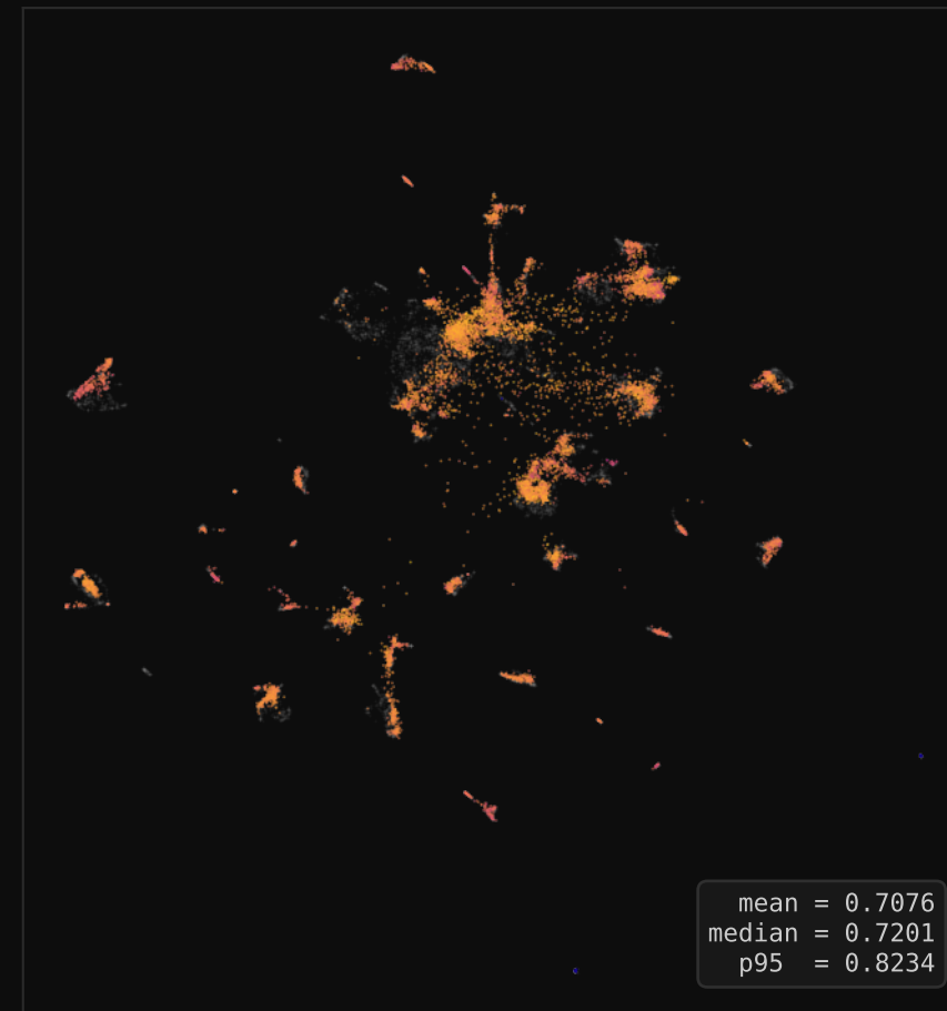
Per-Feature 2-bit
