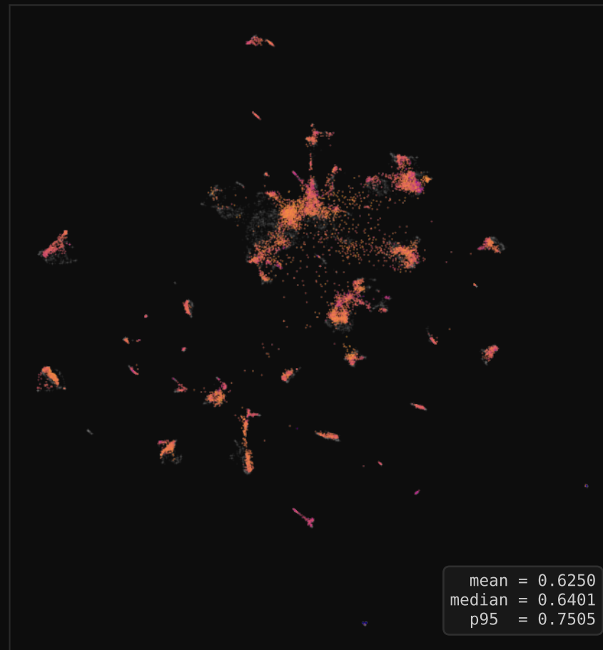
Per-Feature 4-bit
