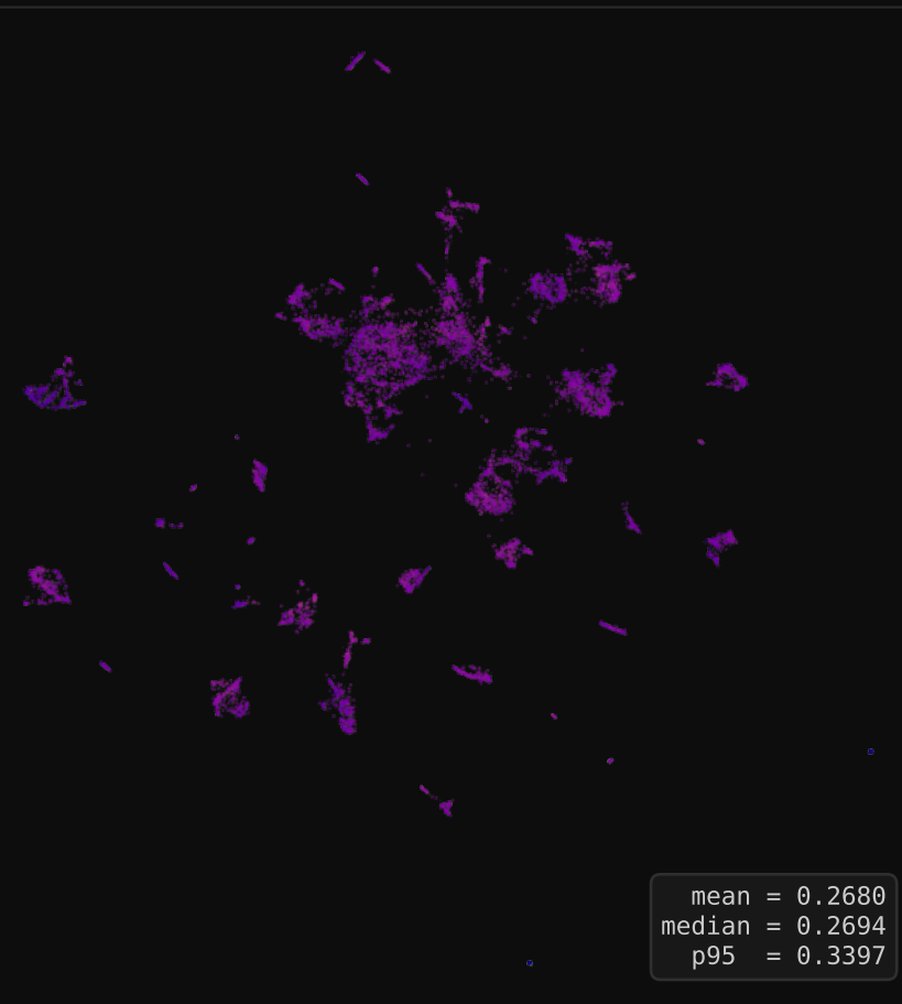
Per-Feature 8-bit
