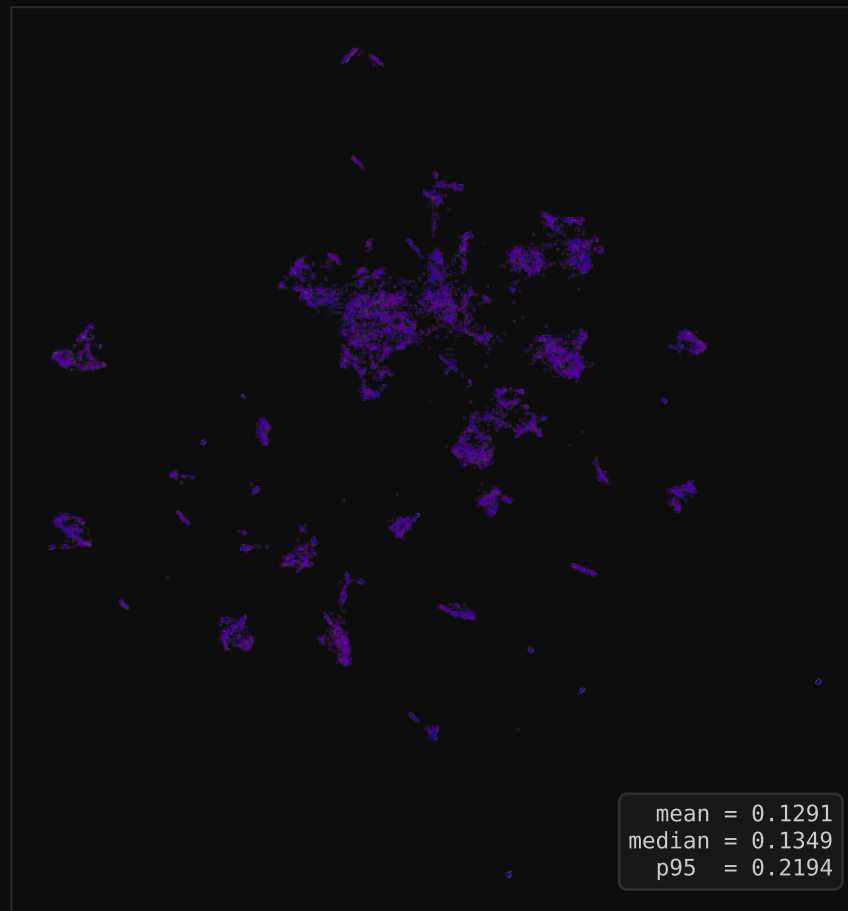
Per-Feature 6-bit
