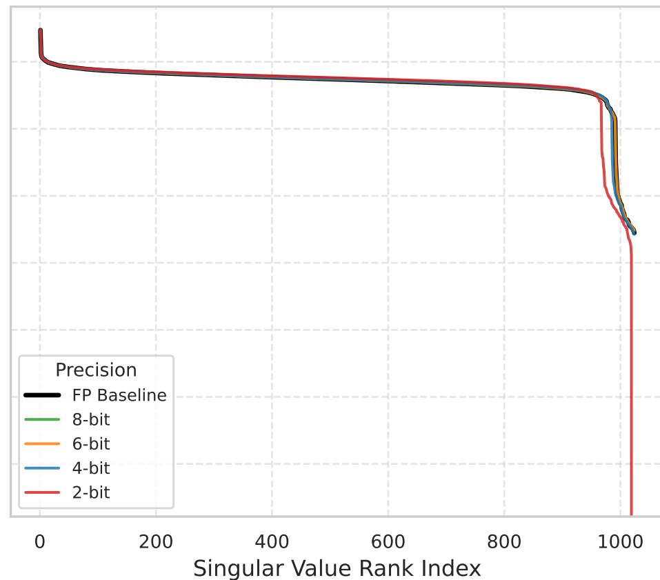
Per-Feature Quantization
