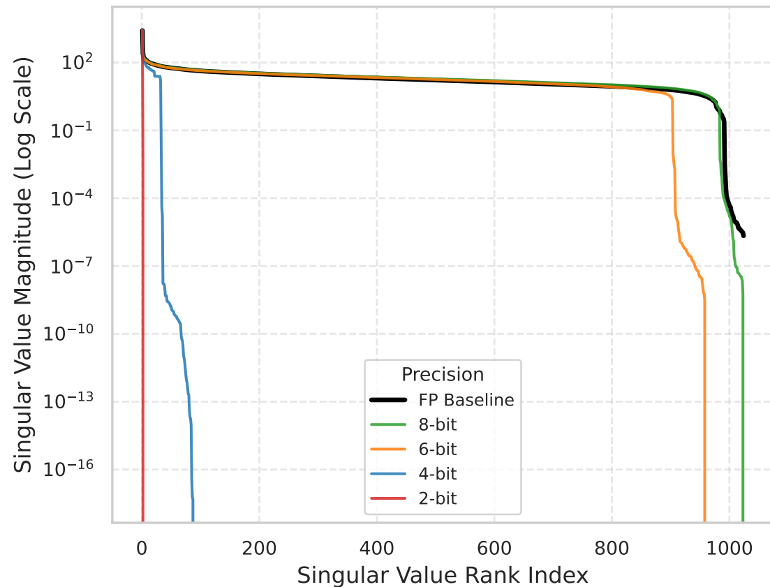
Per-Tensor Quantization
