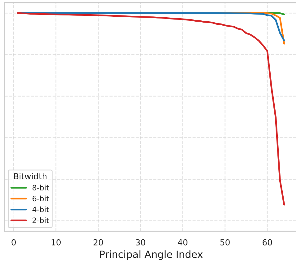
Per-Feature (k=64)
