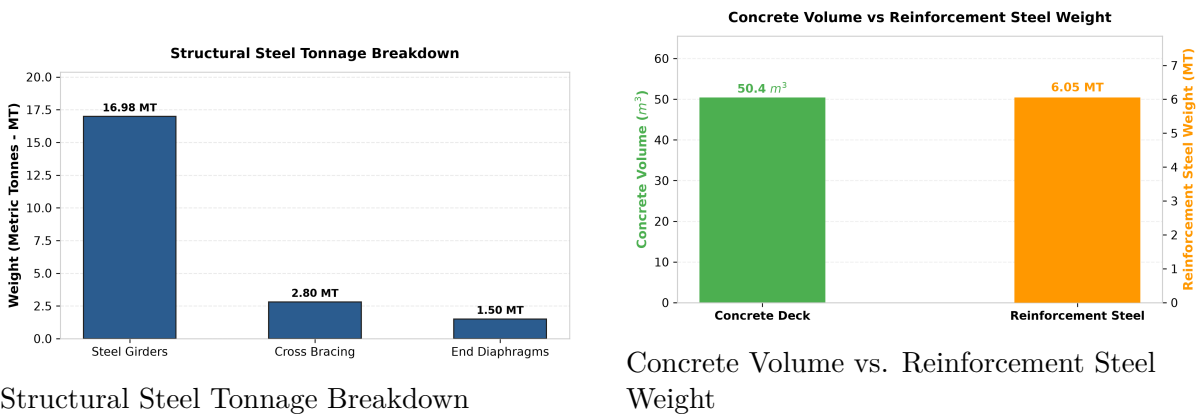
Figure 7.1 – Material Quantity Breakdown Charts
