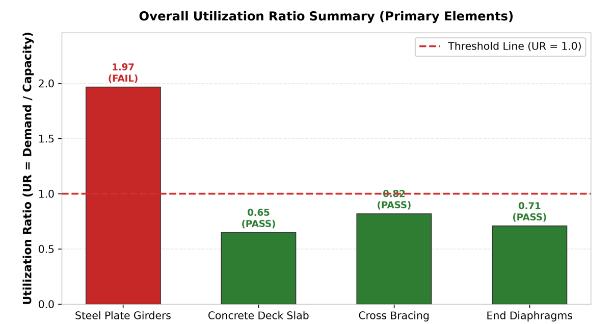
Figure 5.5 – Overall Utilization Ratio (UR = Demand / Capacity) Summary Chart
