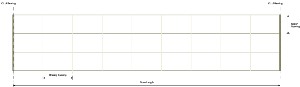
Figure 1 – Overall Bridge Plan
