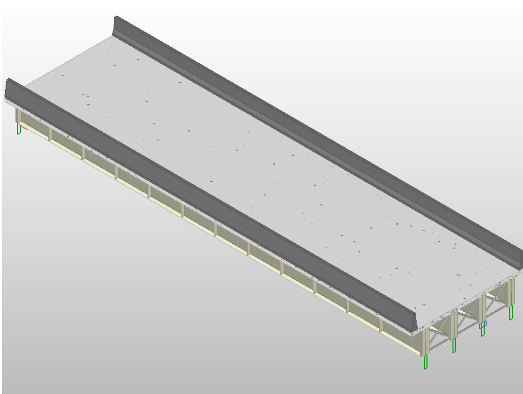
Figure 6.1: Overall 3D Bridge Superstructure
