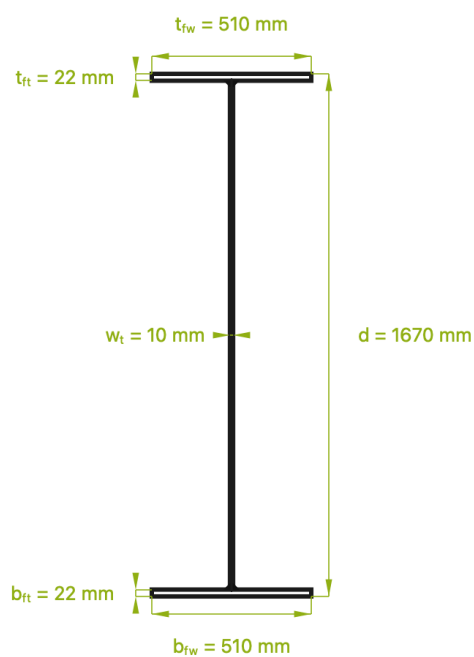
Figure 6.5: Cross Section of Plate Girder
