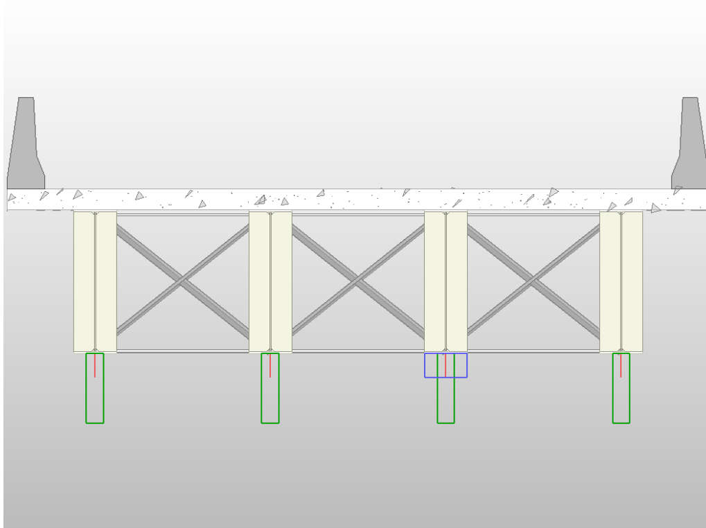
Figure 6.2: Typical Cross Section
