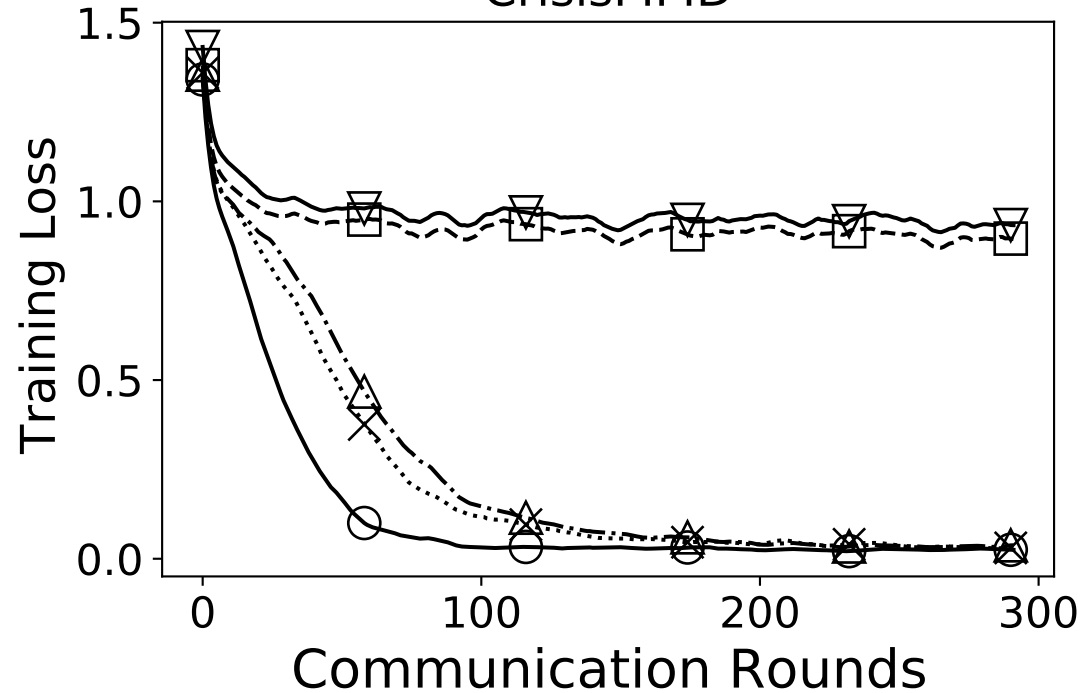
CrisisMMD
