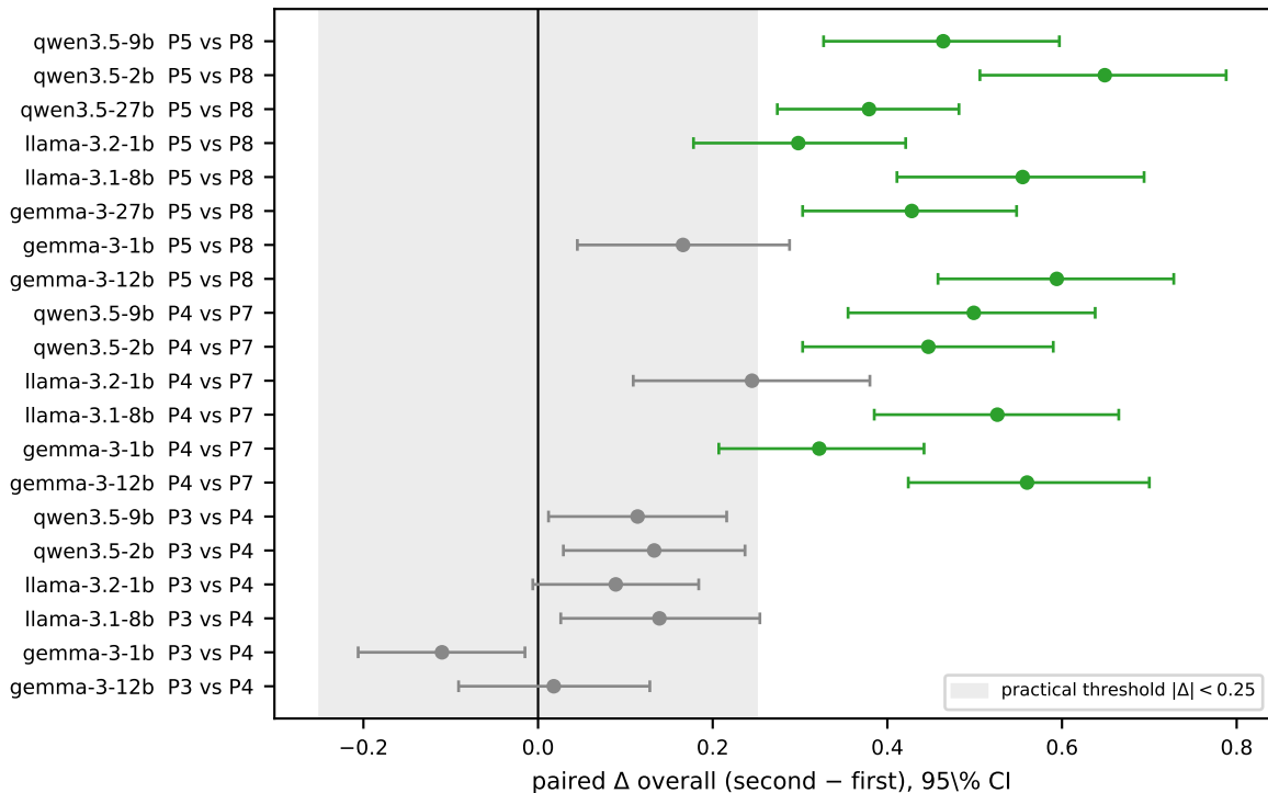
CPT-over-SFT (P3 → P4) and matched RAG effect (P4 → P7, P5 → P8). Green = practically significant
