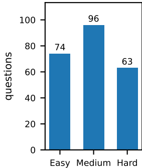
(a) Difficulty
