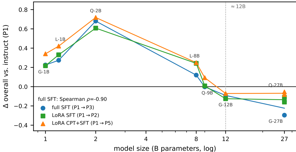
Fine-tuning gain vs. scale
