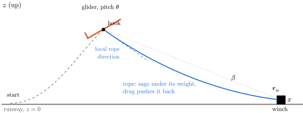
Figure 1: Geometry of a winch launch (not to scale). The glider starts at the left and the winch pulls from the right. The rope sags below the straight line of sight, so at the hook it pulls more steeply downwards than the line to the winch. \beta is the elevation of the glider seen from the winch.
