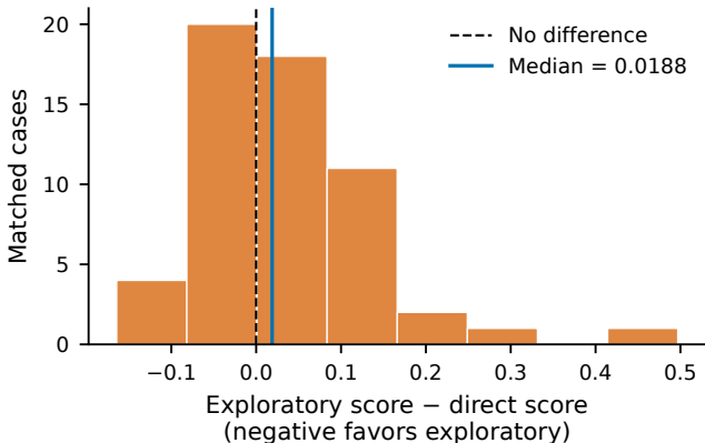
Effect size distribution
