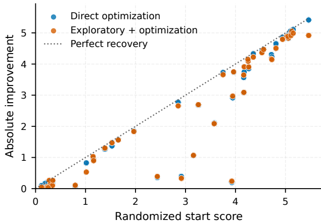
Absolute improvement based on randomized score for exploratory and direct prompt
