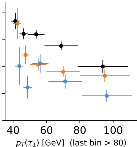
Run2016H, decay mode 1
