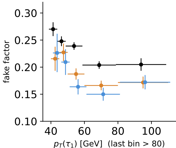
Run2016G, decay mode 1
