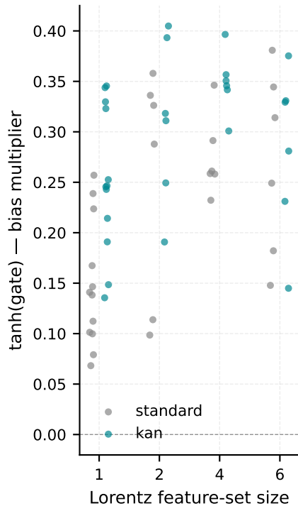
Per-module gate (60 runs)
