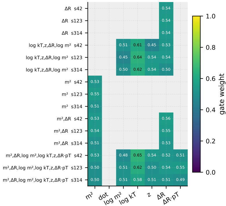
\sigma(\text{feature\_gates}) \cdot \text{KAN, sparse=on}
