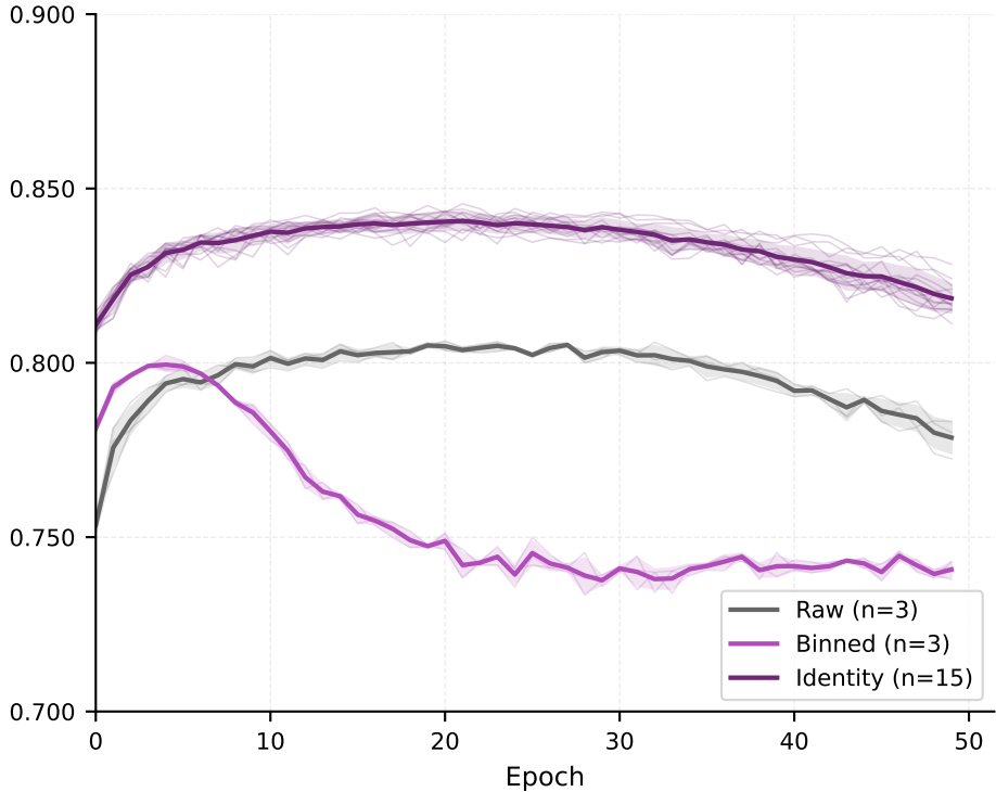
Validation AUROC over epochs
