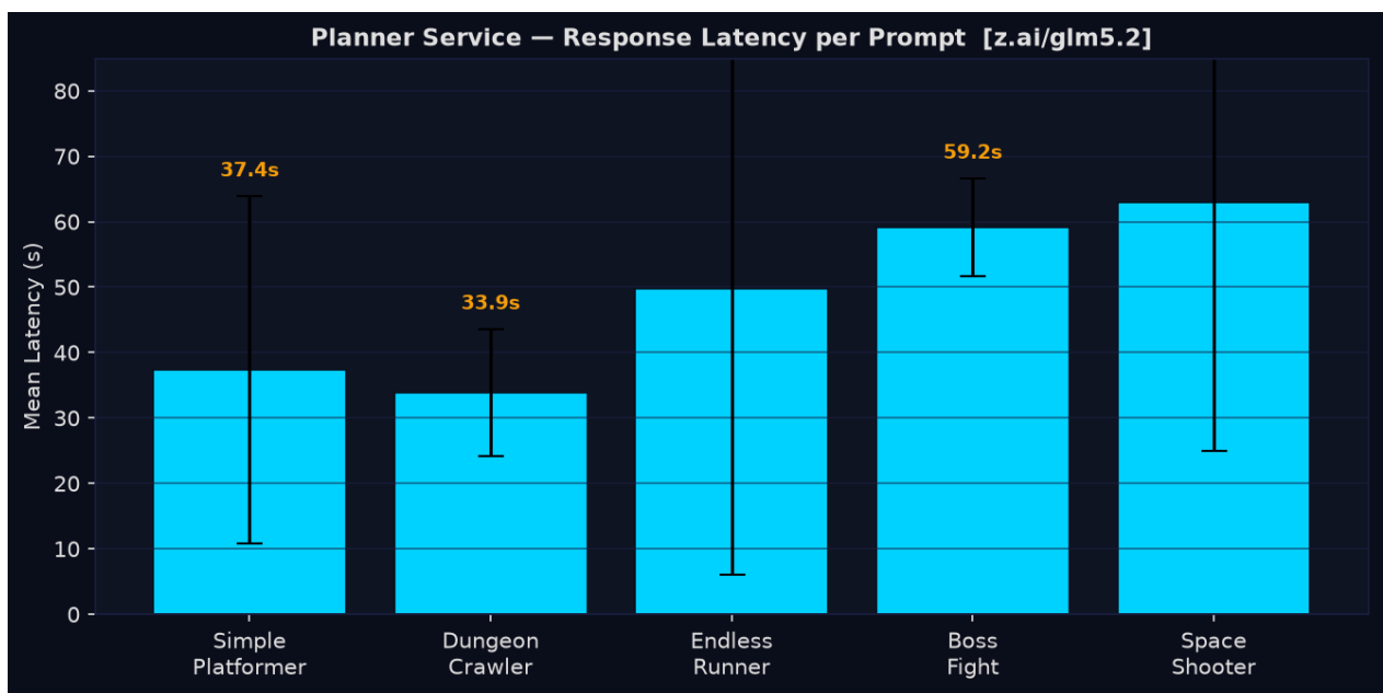
Figure 6.1 — Benchmark Chart: Planner Service Latency
