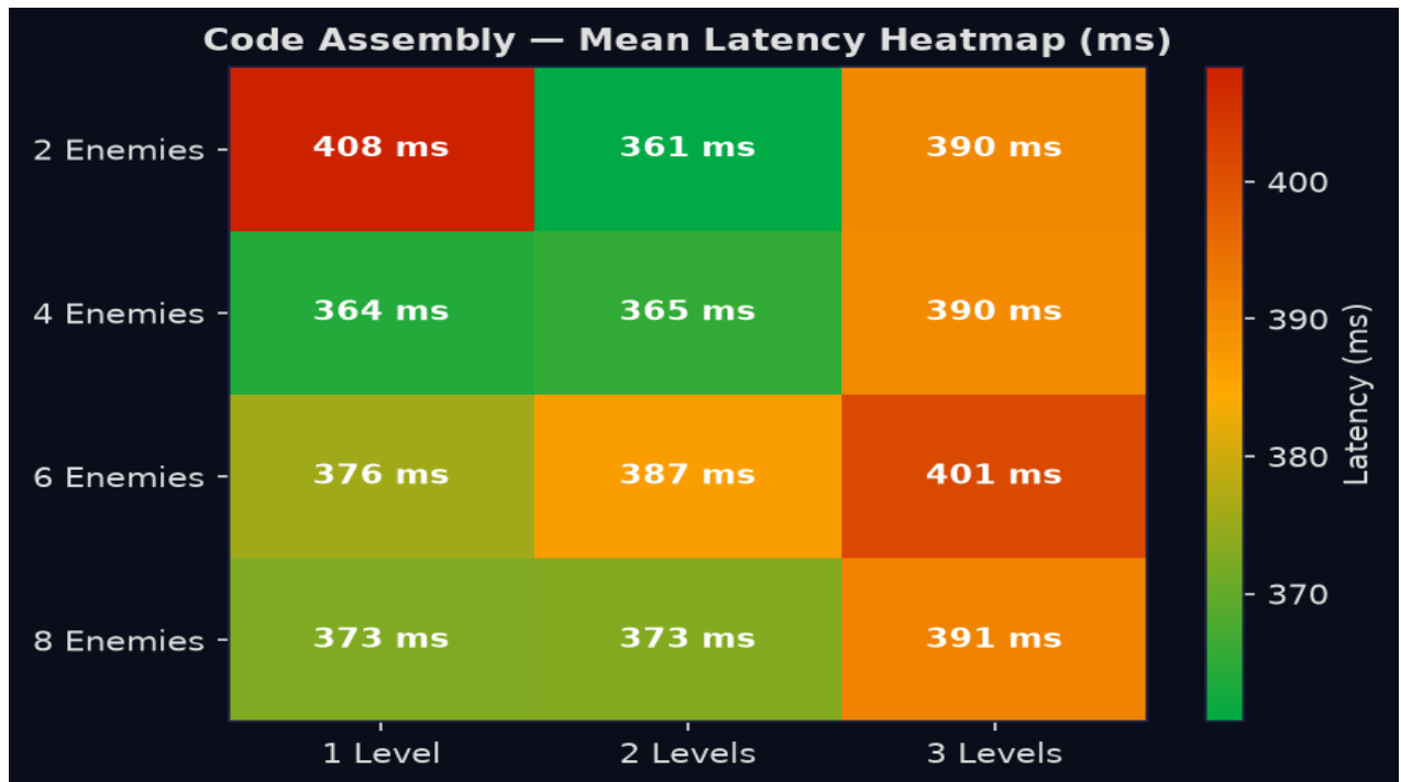
Figure 6.4 — Benchmark Chart: Code Assembly Scaling
