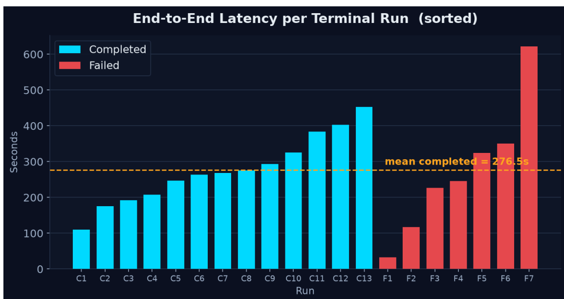
Figure 6.9 — Production: End-to-End Latency per Terminal Run
