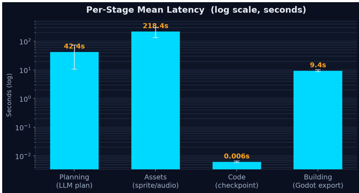
Figure 6.8 — Production: Per-Stage Mean Latency (log scale)
