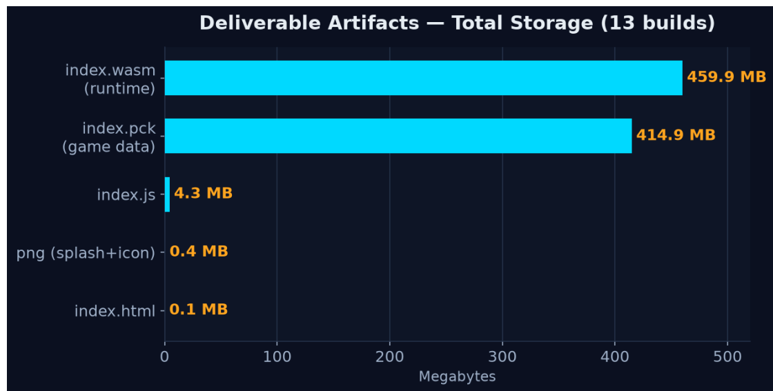
Figure 6.11 — Production: Deliverable Artifacts by Total Storage
