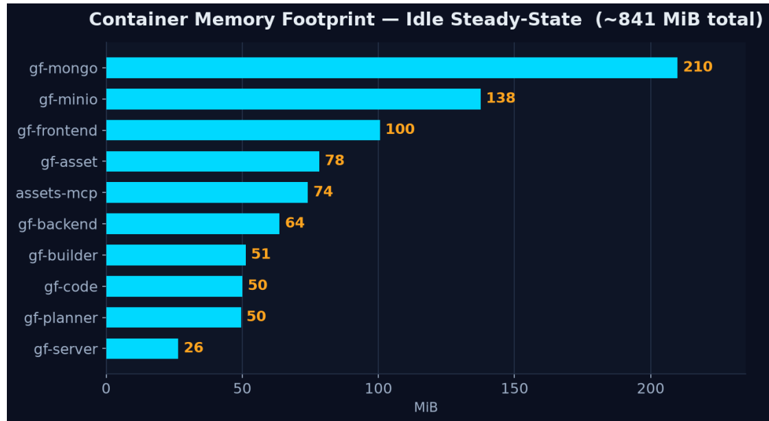
Figure 6.15 — Production: Container Memory Footprint (idle)
