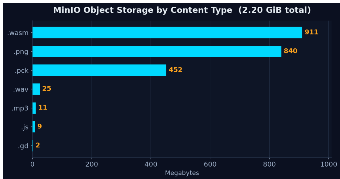
Figure 6.14 — Production: MinIO Object Storage by Content Type
