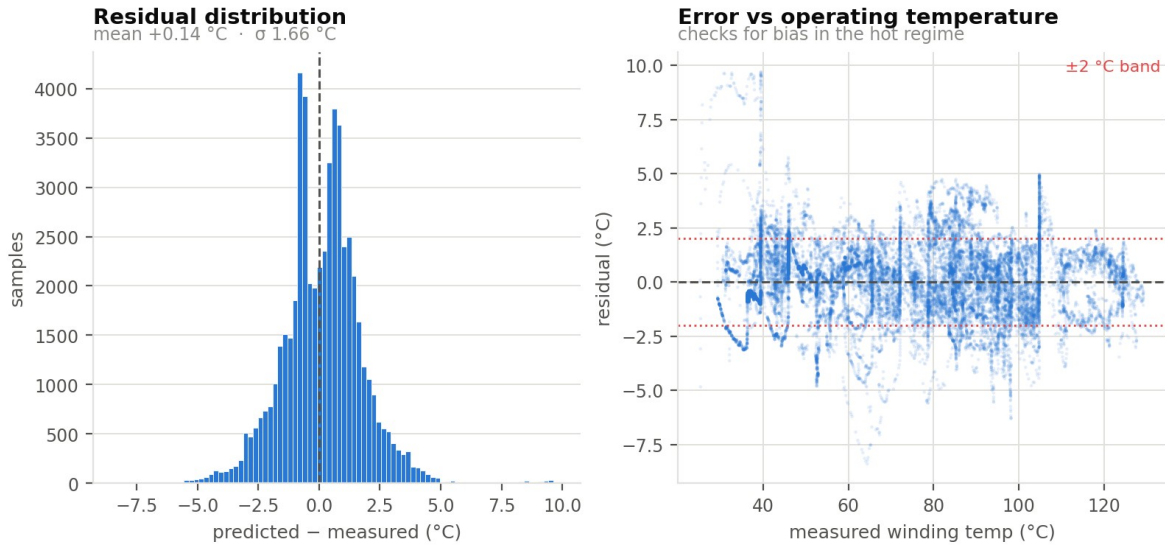
Figure 8 — Residual distribution (left) and residual against measured temperature (right) for the selected model.
