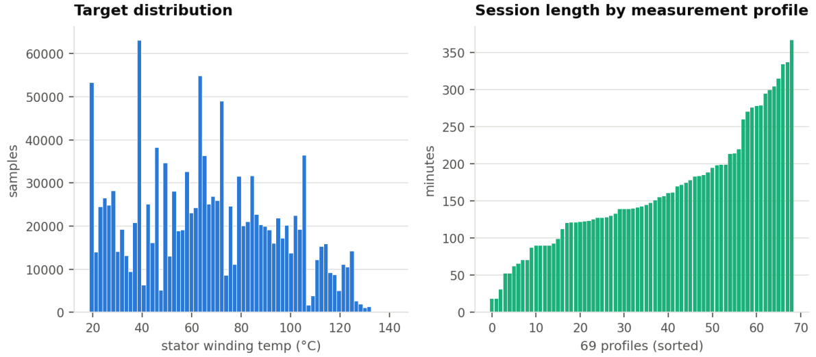
Figure 1 — Dataset structure. Left: the target spans the full range from ambient to near-rated temperature, with no degenerate concentration. Right: session lengths vary from 18 to 366 minutes, which motivates grouping by session rather than by sample.
