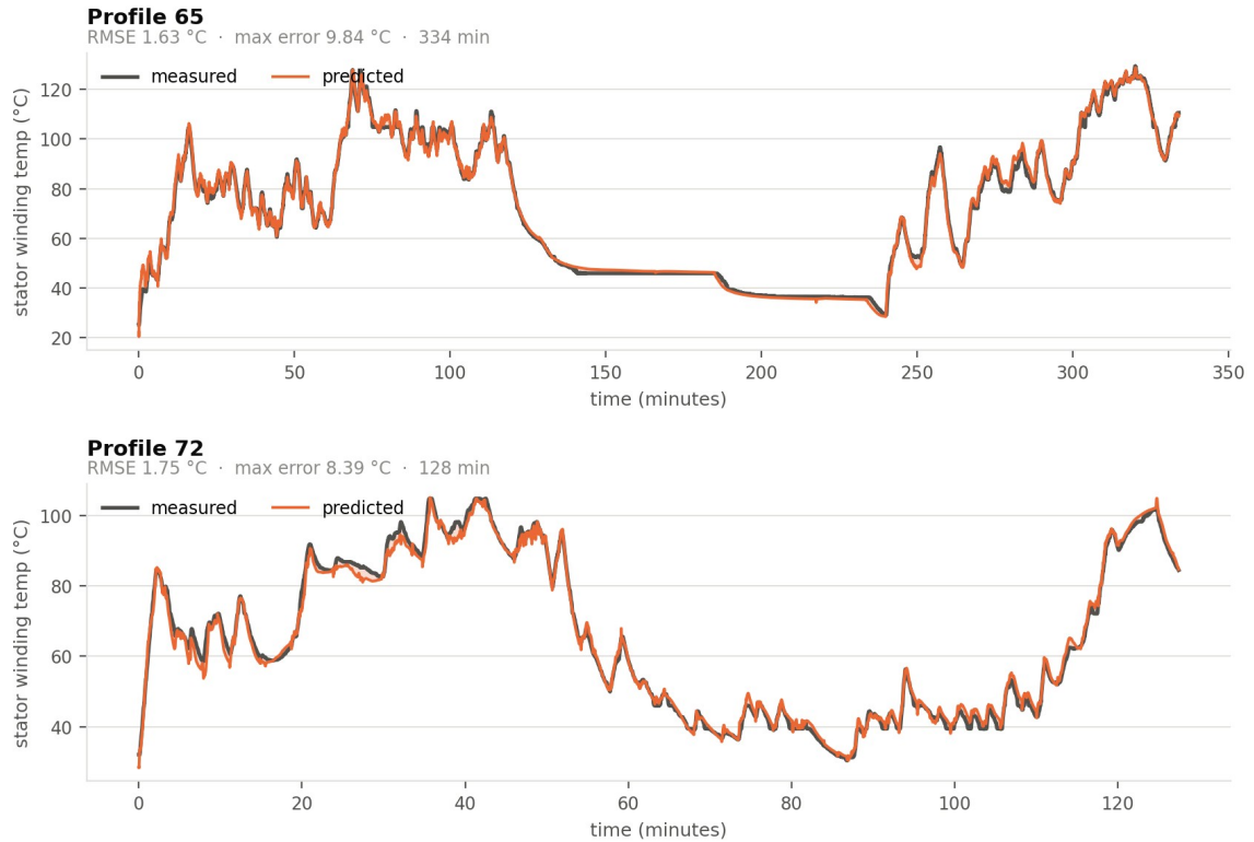
Figure 7 — Selected model (MLP) predicted against measured winding temperature on the two held-out sessions. Neither session was seen in any form during training.
