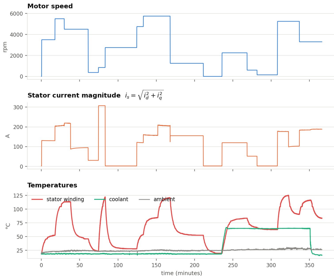
Figure 3 — Electrical excitation versus thermal response, profile 20. Motor speed and current change in seconds; winding temperature responds over minutes and continues to rise after the current has stepped down.
