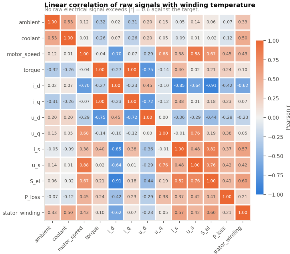
Figure 4 — Pearson correlation between raw and instantaneously-derived signals and the target.
