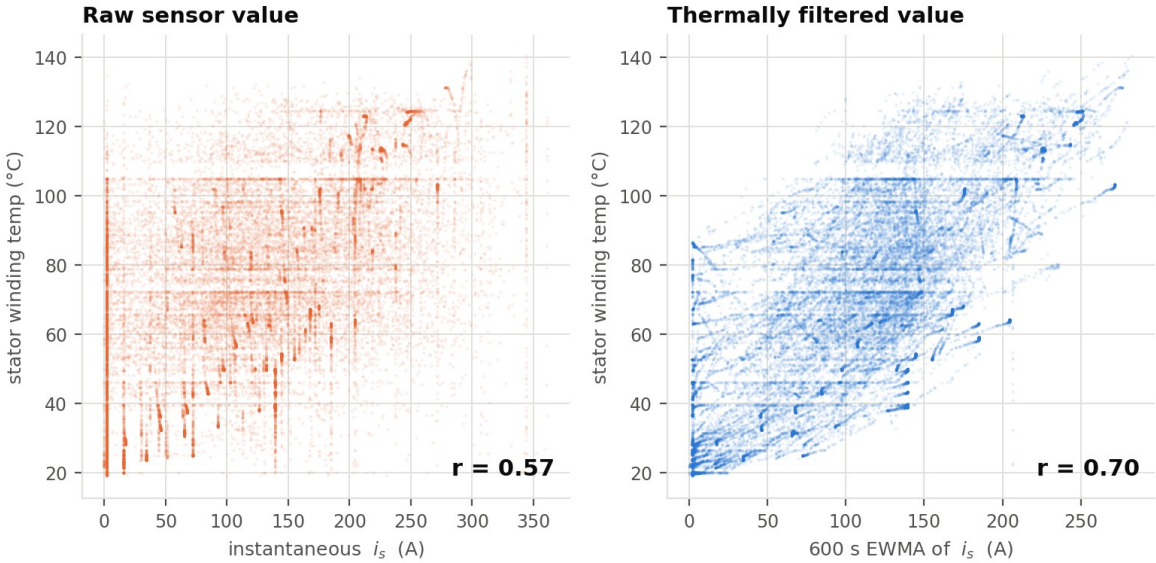
Figure 5 — Instantaneous current magnitude (left) and its 600-second exponentially weighted average (right), each plotted against winding temperature. A single transform raises the correlation from 0.57 to 0.70 and converts a diffuse cloud into a structured relationship.
