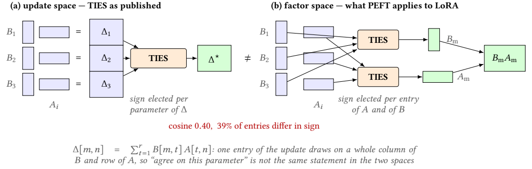
Fig. 2. Sign election in update space and in factor space are different operations. (a) The published algorithm forms each specialist’s update \Delta_i = B_i A_i and elects a sign per parameter of the update . (b) The standard LoRA implementation, and the one we use, applies the same rule independently to the A factors and to the B factors and multiplies the results, so signs are elected per factor entry . Because each entry of \Delta is a sum over the rank, no factor entry corresponds to one parameter of the update, and the two merges do not coincide: on random factors at r=4 with three specialists and density 0.5 their outputs have cosine similarity 0.40 and disagree in sign on 39% of entries. We use (b) because the alternative — assembling \Delta , merging, and re-extracting by SVD — changes the adapter’s rank and adds reconstruction error before the merging rule is evaluated.
