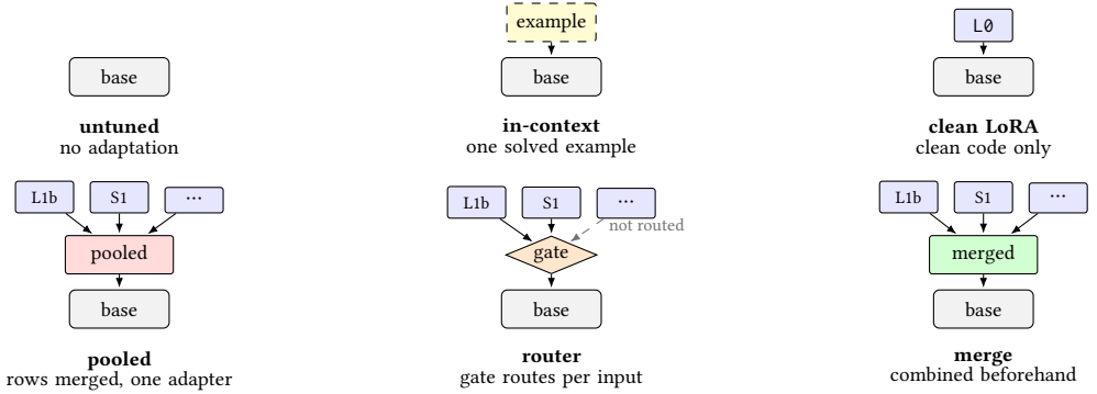
Fig. 3. The six arms. All are the same base model at the same LoRA rank, differing only in how the training data is used and where per-transform knowledge is combined. Top row: arms that never see an obfuscated program in training — untuned , in-context , and the clean LoRA control that separates learning the task from learning the transforms. Bottom row: the three ways to spend the obfuscated data. The labelled boxes are the six training conditions, named by obfuscator (L1b, S1, and four more); all three arms receive the same six. In the router panel the dashed path marks an expert the gate does not select for a given input; the merge combines all of them unconditionally. The three are ordered by when the conditions are combined — pooled collapses them during training, router composes them per input at inference and must keep every expert resident, and merge composes them in weight space beforehand, leaving one adapter with no gate and no run-time cost. The KL-consistency arm is pooled with an added consistency term (Section 5).
