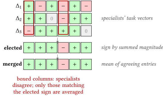
Fig. 2. Sign-consensus merging, on six parameters of three specialists. Each specialist contributes a task vector — the update its own training produced. Averaging these directly lets disagreeing updates cancel. TIES instead trims small entries, elects a sign per parameter by summing signed magnitudes across specialists, and averages only the entries that match it, so a parameter two specialists push positive and one pushes negative is merged from the two (boxed columns) [20]. DARE-TIES prepends a random drop of a fraction of each vector's entries with rescaling of the survivors, preserving the update in expectation [21]. Nothing is trained: both are arithmetic on weights already learned, and the result is one adapter of the original rank.
