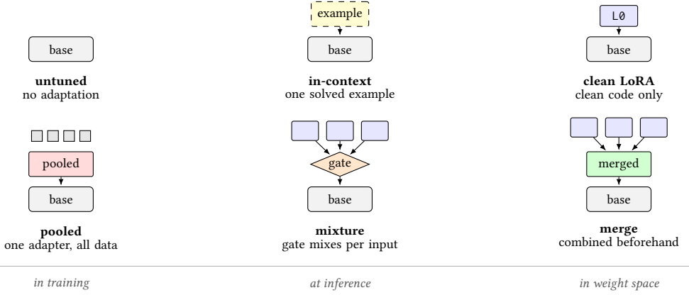
Fig. 1. The six arms. All are the same base model at the same LoRA rank, differing only in how the training data is used and where per-transform knowledge is combined. Top row: arms that never see an obfuscated program in training — untuned , in-context , and the clean LoRA control that separates learning the task from learning the transforms. Bottom row: the three ways to spend the obfuscated data, ordered by when the specialists are combined — pooled collapses them during training, mixture composes them per input at inference and must keep every expert resident, and merge composes them in weight space beforehand, leaving one adapter with no gate and no run-time cost. The anchored objective is pooled with an added consistency term (Section 2.4).
