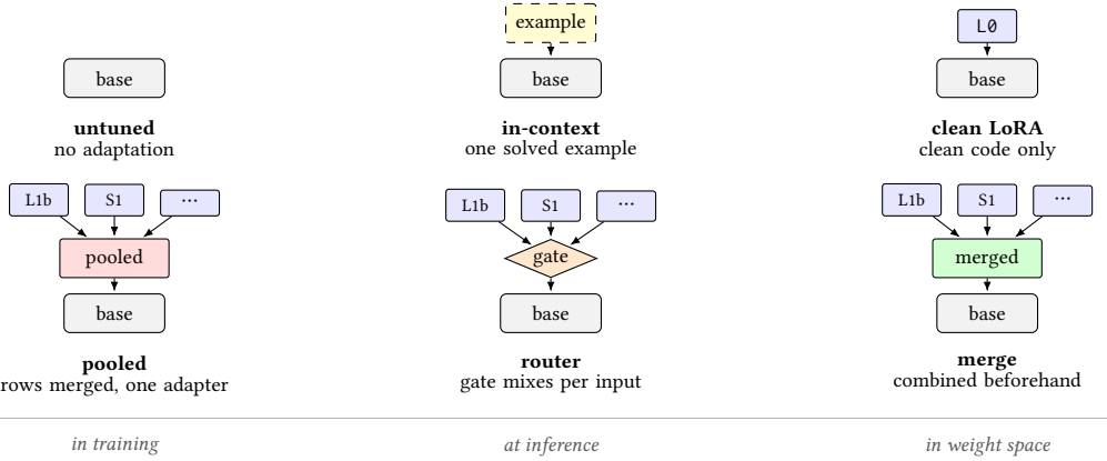
Fig. 3. The six arms. All are the same base model at the same LoRA rank, differing only in how the training data is used and where per-transform knowledge is combined. Top row: arms that never see an obfuscated program in training — untuned , in-context , and the clean LoRA control that separates learning the task from learning the transforms. Bottom row: the three ways to spend the obfuscated data. The labelled boxes are the six training conditions, named by obfuscator (L1b, S1, and four more); all three arms receive the same six. They are ordered by when those are combined — pooled collapses them during training, router composes them per input at inference and must keep every expert resident, and merge composes them in weight space beforehand, leaving one adapter with no gate and no run-time cost. The KL-consistency arm is pooled with an added consistency term (Section 5).
