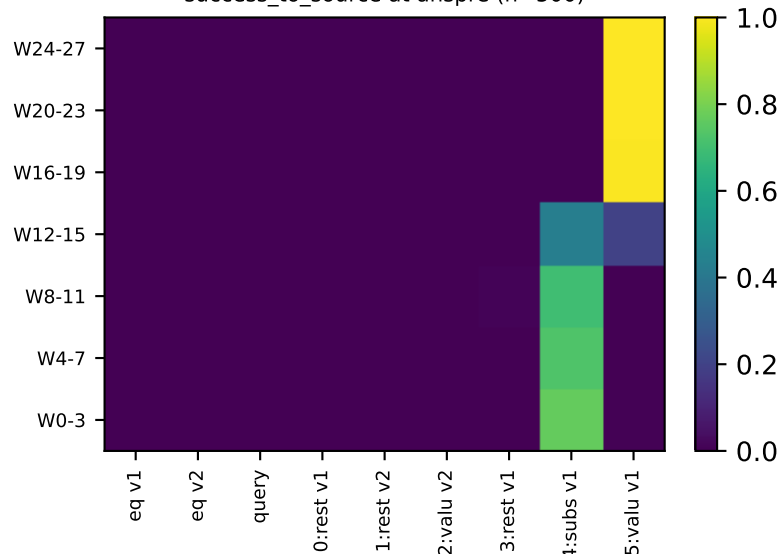
source: other success_to_source at anspre (n=500)
