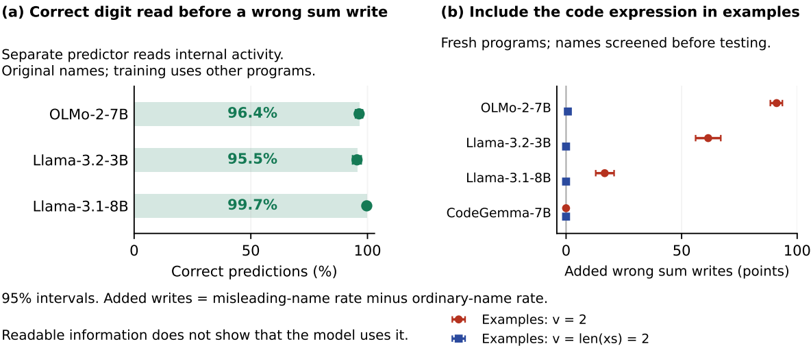
Figure 2: (a) Correct-digit readout before wrong sum writes. (b) Example-format effects on fresh programs with screened names.
