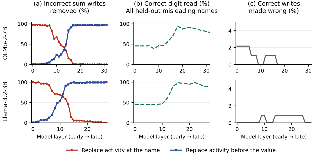
Figure 3: (a) Name-error removal. (b) Correct-digit readout. (c) Damage to correct writes. Patches use ordinary-name twins.
