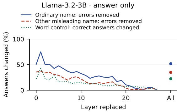
Figure 2: Llama-3.2-3B name-site patches, queried variable, set 7. Removal includes any other digit; All replaces every layer.
