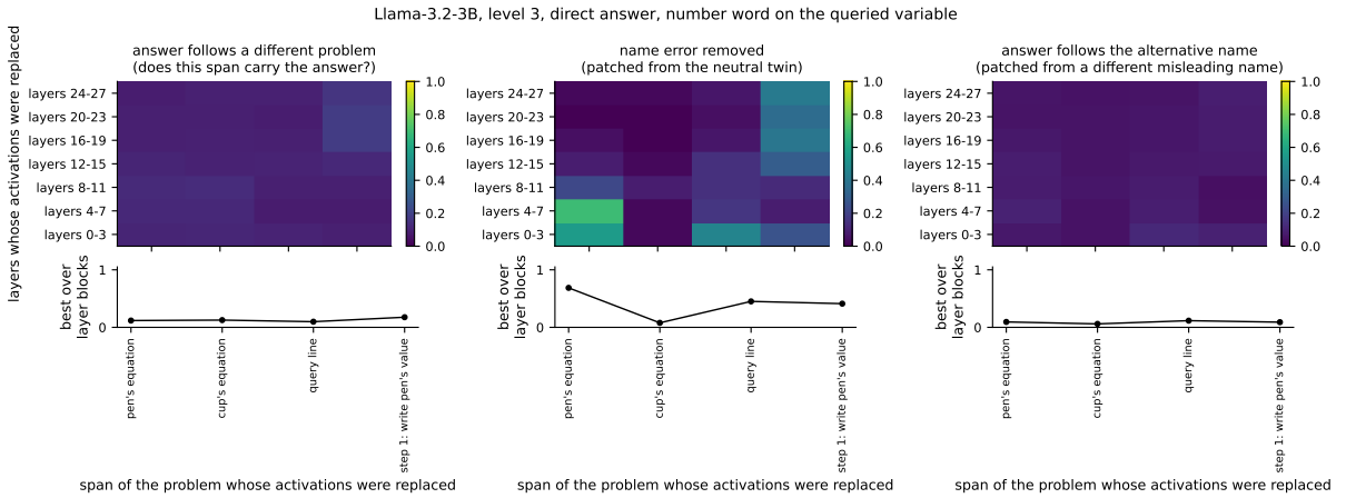
Figure 4: Llama-3.2-3B answer-only patches in four-layer windows. Bottom: maximum over windows.
