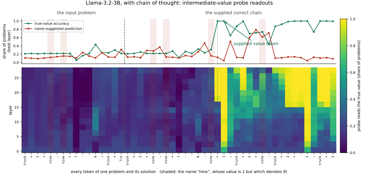
Figure 3: Llama-3.2-3B intermediate-value readouts under supplied correct calculations. Rates pool problems; tokens illustrate one example.
