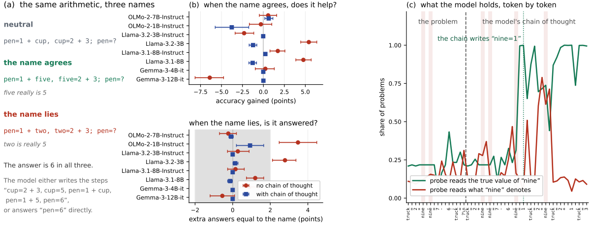
Figure 1: (a) The manipulation: one problem, three names for the same variable, one answer. (b) What the name does to the answer, for each model, at level 3, averaged over three sets of worked examples; bars are 95% bootstrap intervals over problems. Without a chain of thought (red) a name that agrees with the value adds accuracy and a name that lies is answered in its place. With a chain of thought (blue) neither happens: every model sits inside the two-point band we fixed in advance as the largest effect we would call meaningful. (c) Inside the model, at every token of one problem: a probe trained only on neutral problems reads the lure at the name’s own tokens (shaded) and nowhere else, and stops reading it the moment the chain writes the variable’s value.
