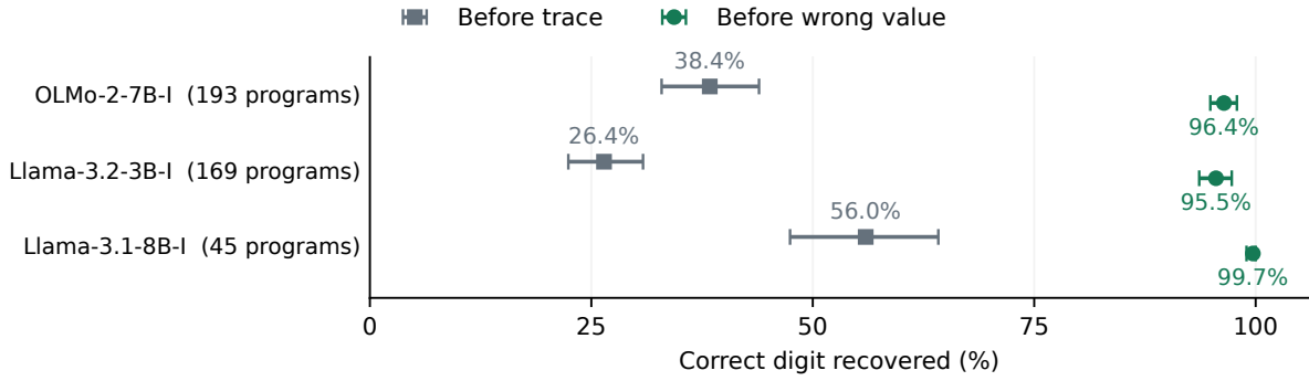
Figure 2: Correct-digit recovery at both positions on the same eventual name-suggested error cases (95% intervals). Counts are unique programs. I: instruction-tuned.
