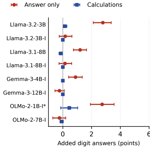
(a) Arithmetic, queried variable
