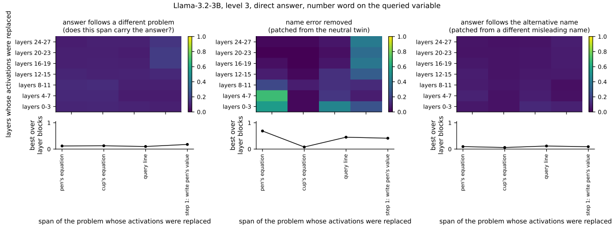
Figure 6: Llama-3.2-3B answer-only patches in four-layer windows. Bottom: maximum over windows.
