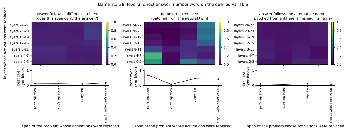
Figure 29: The same grids in the direct regime, queried variable.
