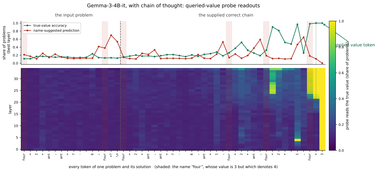
Figure 7: Gemma-3-4B-Instruct, queried variable, misleading-name problems under the correct chain. Top: maximum-over-layers true-value accuracy and name-suggested prediction rate; bottom: true-value accuracy by layer. Shading marks the variable's name; the dotted line marks the position before its value; the arrow marks the supplied digit itself.
