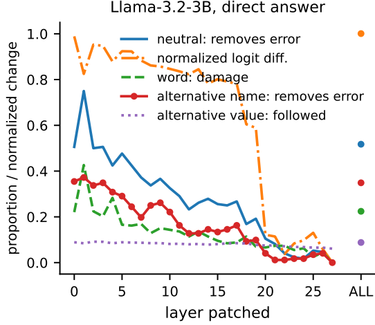
Figure 3: Llama-3.2-3B, answer-only: queried-variable name errors removed by layer, with neutral-word damage and alternative-name controls. Removal counts changes away from the name-suggested digit.
