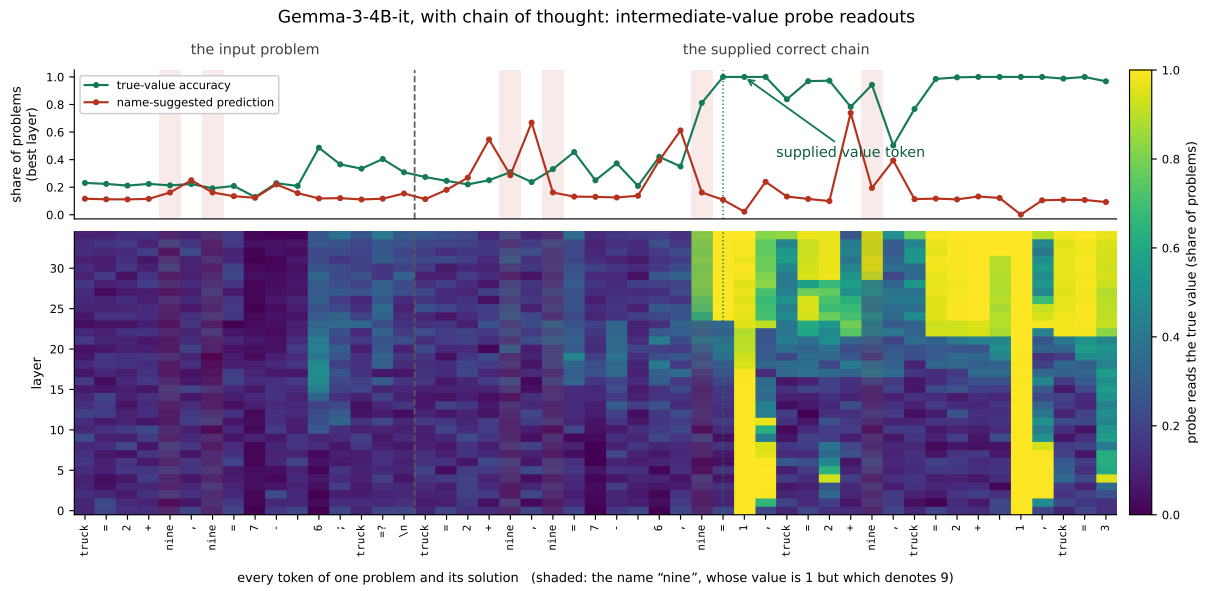
Figure 8: The same Gemma token sweep for the intermediate variable. Both figures use neutral-trained probes; no misleading-name problems enter training.
