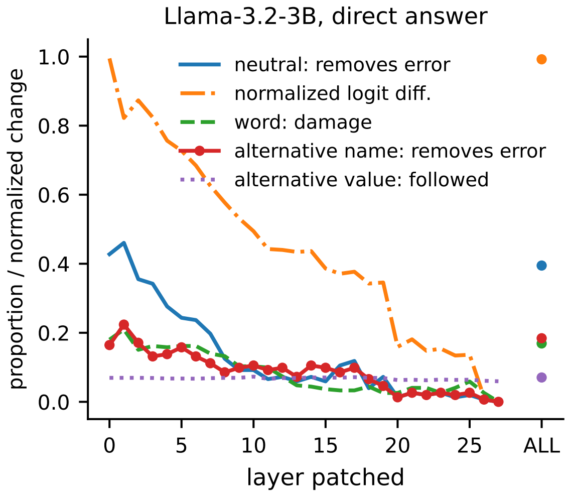
Figure 25: Name errors removed by patching, by layer, with both controls.
