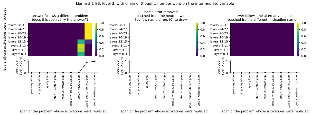
Figure 36: Llama-3.1-8B, span-by-layer-window patching grids, chain-of-thought regime. The error-removal panel is empty: none of the 500 patched problems is answered with the name-suggested value.
