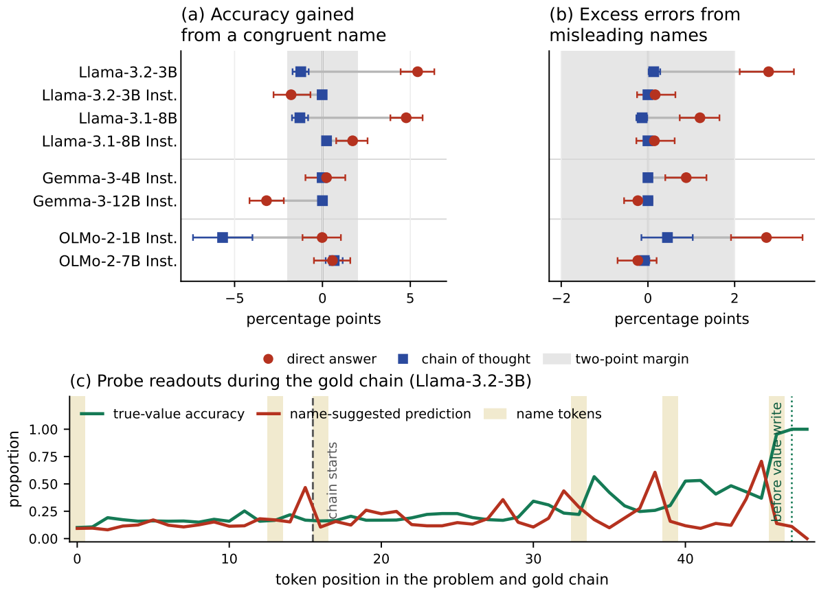
Figure 9: Queried-variable effects at level 3: congruent-name accuracy gains, excess name errors, and best-layer correct-calculation readouts. Bars: 95% intervals; grey: a two-point reference band. OLMo-2-1B is below the planned accuracy floor.
