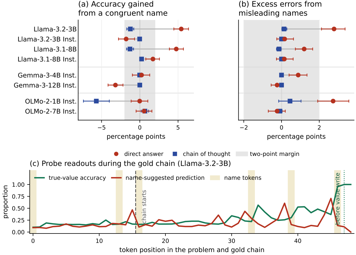
Figure 2: Level 3 queried-variable effects: (a) congruent-name accuracy gains; (b) excess name errors. Means and 95% intervals across three demonstration sets; grey: \pm 2 points, a reference band rather than an equivalence test. (c) Best-layer true-value accuracy and name-suggested predictions under a supplied correct calculation. OLMo-2-1B is below the planned neutral-accuracy floor. Shading: name positions; dotted line: position before the queried value.
