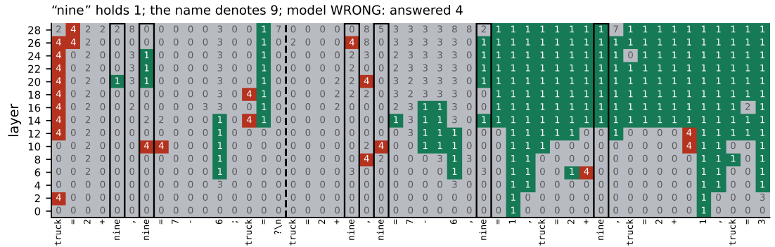
Figure 19: Intermediate-variable example from a problem answered wrongly. Red is the model’s final answer, which is the queried variable’s value, so a cell that matches it is not a readout of this variable.
