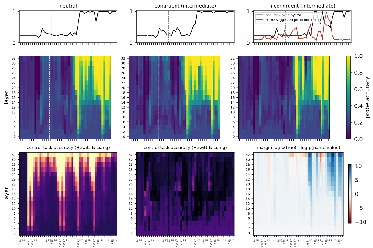
Figure 34: Llama-3.1-8B, chain-of-thought regime, intermediate variable.
