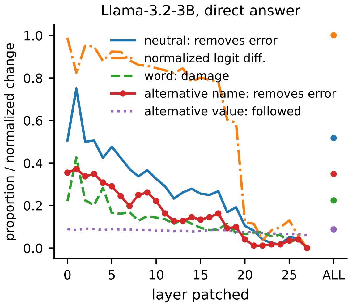
Figure 30: Name errors removed by patching, by layer, with both controls, queried variable.
