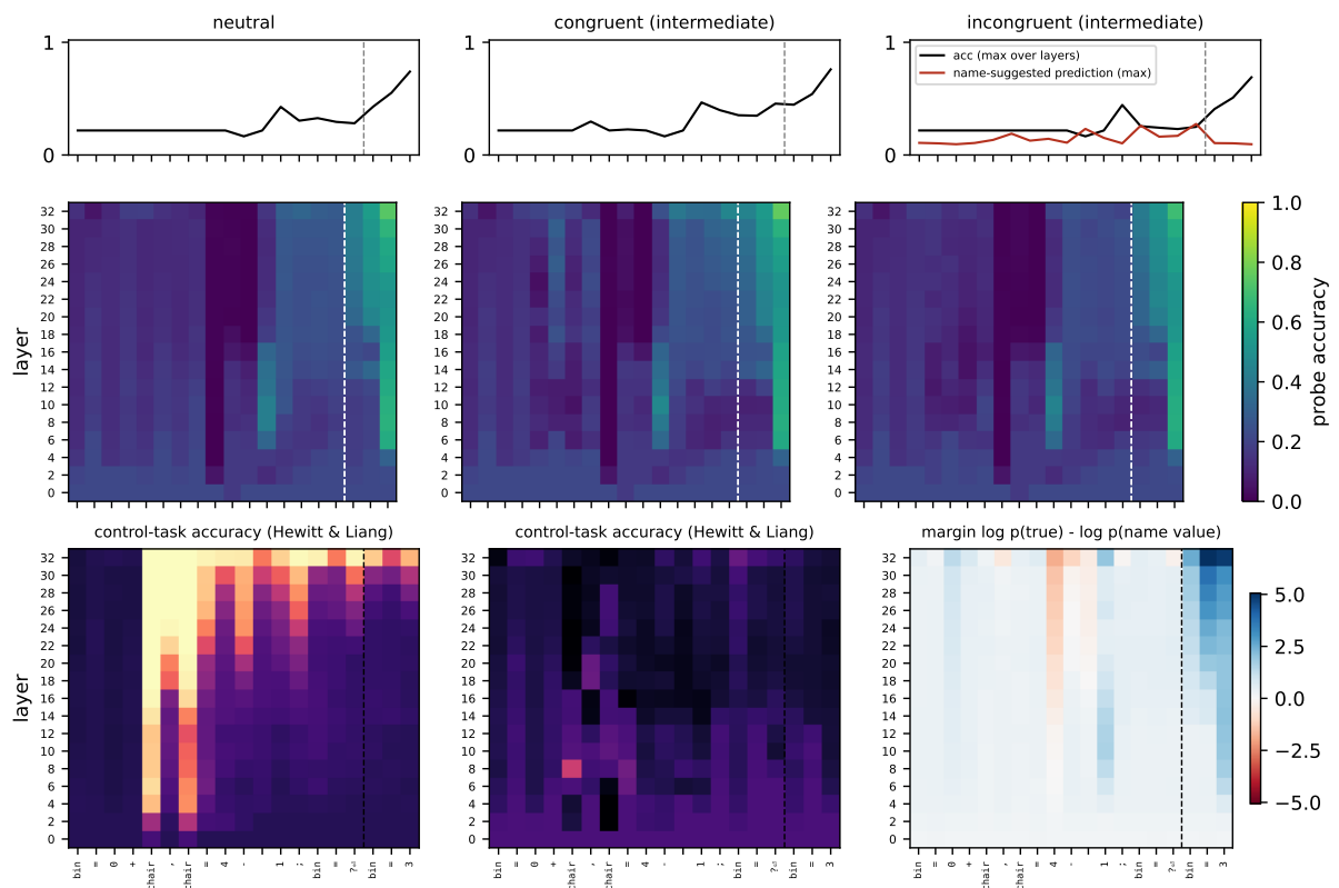
Figure 35: Llama-3.1-8B, direct regime, intermediate variable.
