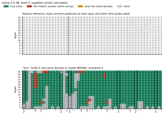
Figure 5: Correct-calculation probe predictions for a problem answered with the name-suggested digit. Top: neutral modal prediction (one seed); bottom: majority prediction (three seeds). Green: true value; red: wrong answer; amber: name-suggested value; grey: other.
