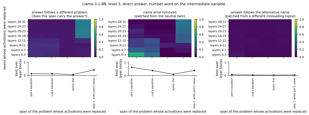
Figure 37: Llama-3.1-8B, the same grids in the direct regime.
