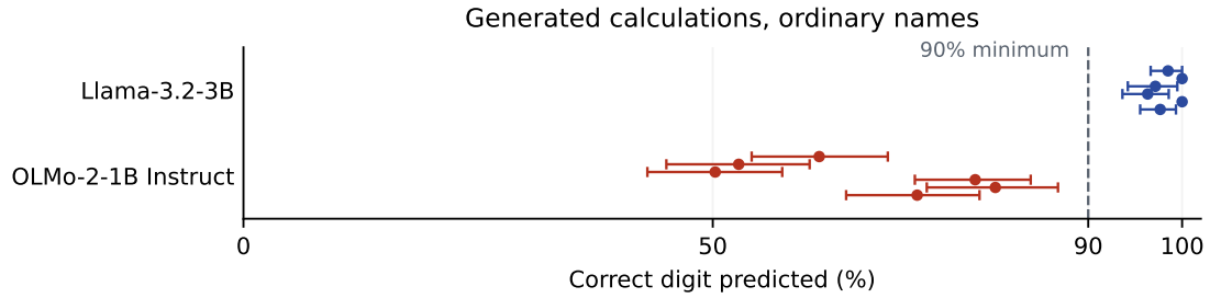
Figure 41: Correct-digit probes on ordinary-name generated calculations: two variables and three demonstration sets per model. Bars: 95% intervals; dashed line: the planned 90% calibration minimum.
