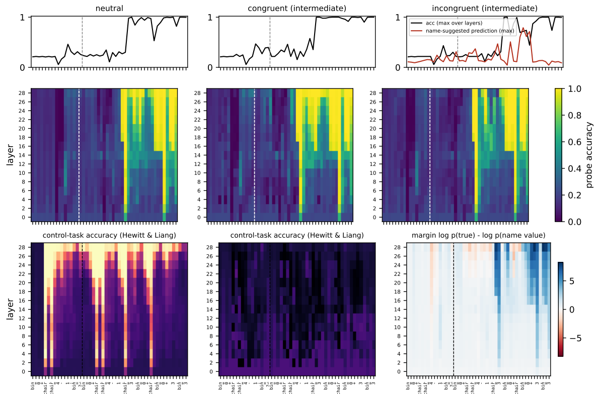
Figure 21: Accuracy heatmaps by token and layer for the neutral, congruent and incongruent conditions, in the layout of Kudo et al.'s Figure 2.
