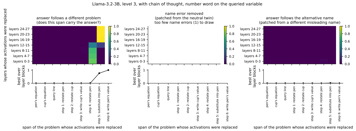
Figure 28: Span-by-layer-window patching grids, chain-of-thought regime, queried variable; the error-removal panel is empty for the same reason.
