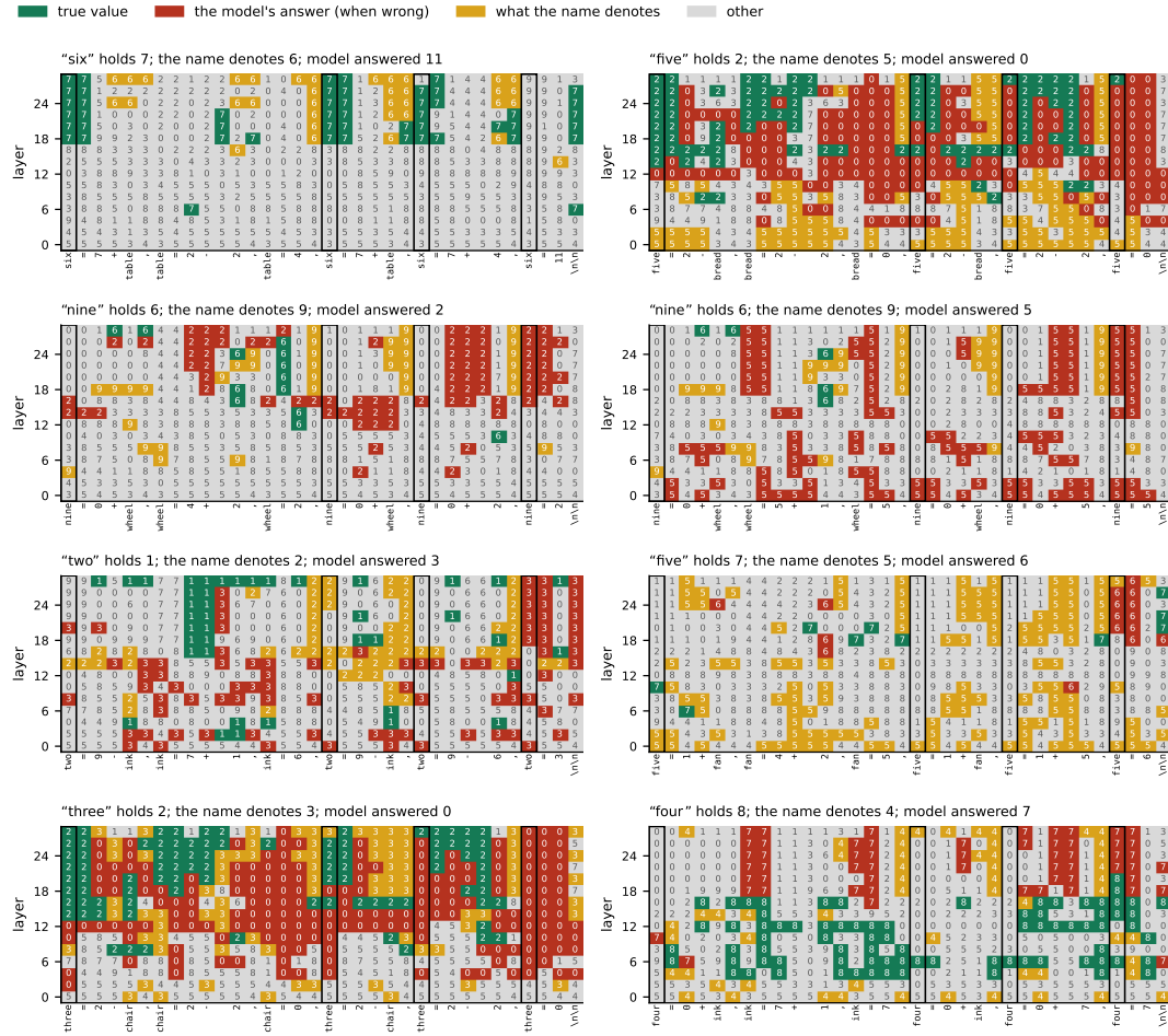
Figure 6: Value-step probes applied to Llama-3.2-3B's generated calculations on the first 8 of 108 incorrectly answered problems. Each panel is one problem; colours follow the legend. Training uses supplied correct calculations on ordinary-name problems.
