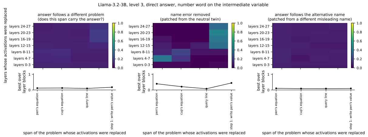
Figure 24: The same grids in the direct regime.
