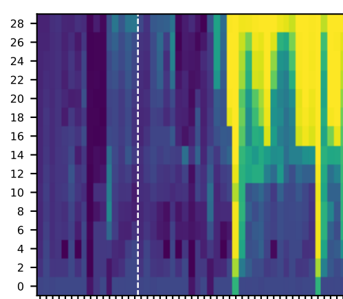
control-task accuracy (Hewitt & Liang)
