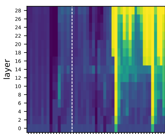
control-task accuracy (Hewitt & Liang)
