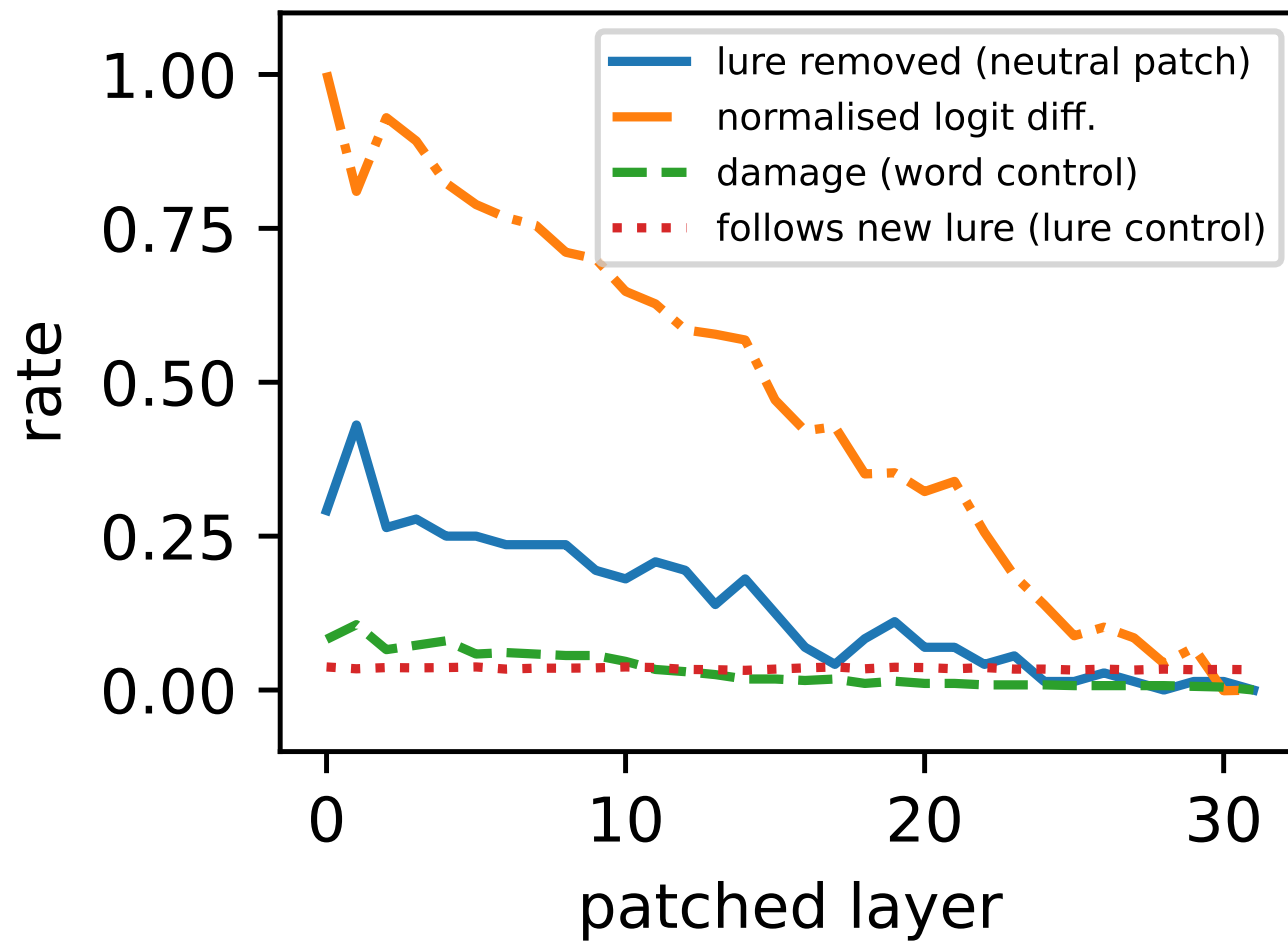
Figure 28: fig3_patching_llama31-8b_L3_v2.
