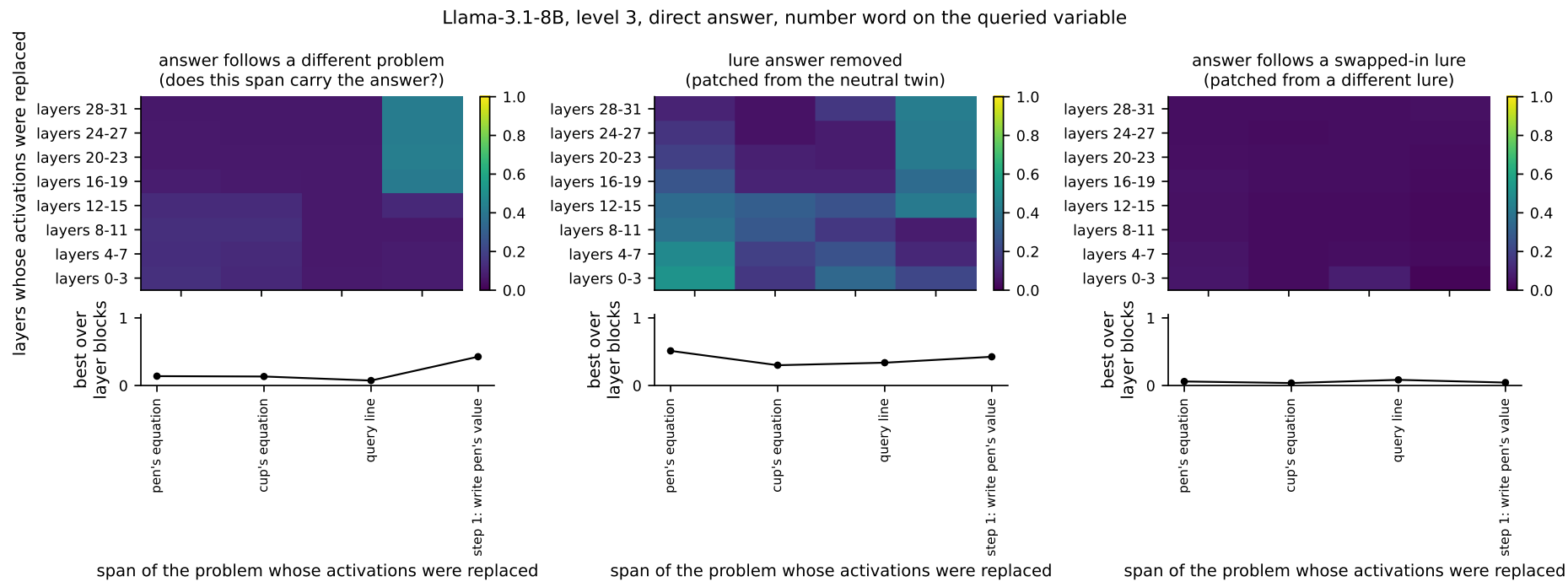
Figure 35: kudo_fig5_llama31-8b_L3_direct_v1.
