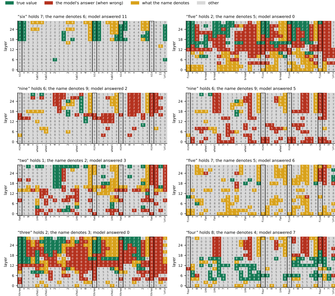
Figure 30: fig_own_chain_llama32-3b_L3_cot_v1.
