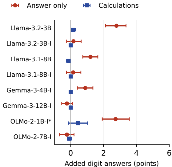
(a) Arithmetic, queried variable
