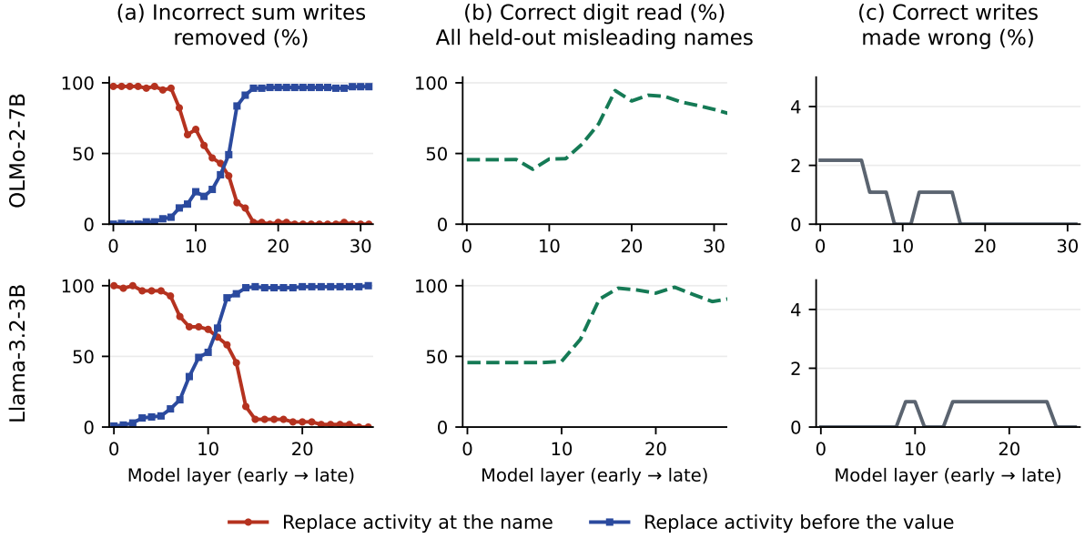
Figure 7: (a) Name-error removal. (b) Correct-digit readout. (c) Damage to correct writes. Patches use ordinary-name twins.
