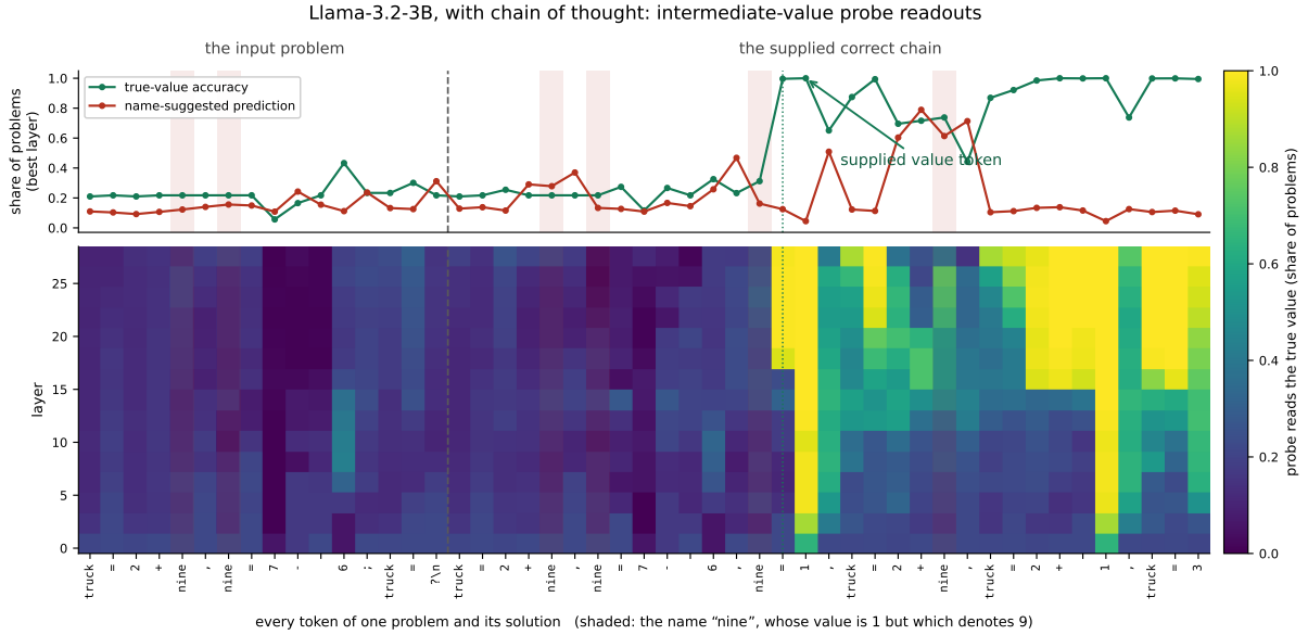
Figure 4: Llama-3.2-3B intermediate-value readouts under supplied correct calculations. Rates pool problems; tokens illustrate one example.
