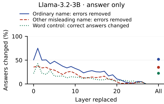
Figure 6: Arithmetic name-site patches, Llama-3.2-3B, queried variable, set 7. All replaces every layer.
