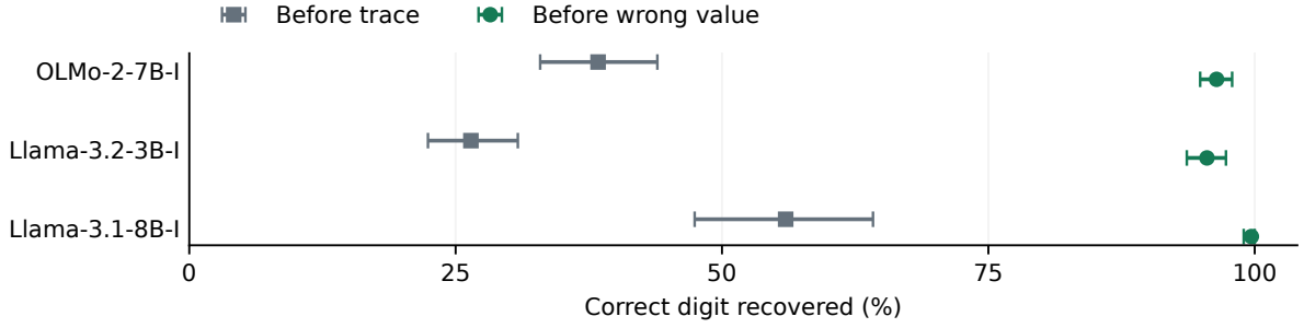
Figure 3: Correct-digit readouts on the same wrong writes (95% intervals). I: instruction-tuned.
