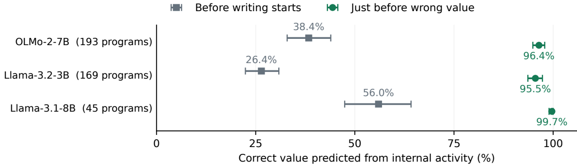
Figure 2: Predictor accuracy on the same eventual errors at both positions (95% intervals). Counts are unique programs.
