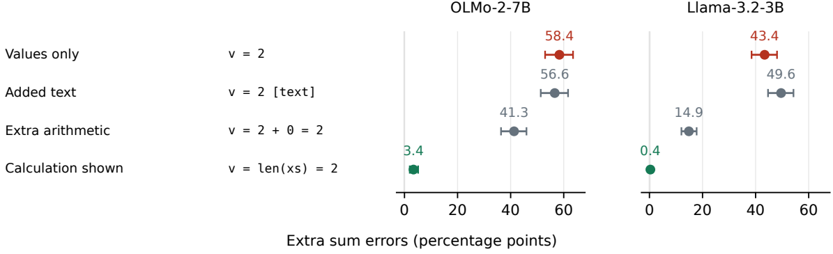
Figure 3: Sum errors report a list’s sum instead of its length. Rates subtract the ordinary-name baseline; bars show 95% intervals. [text]: added filler words.
