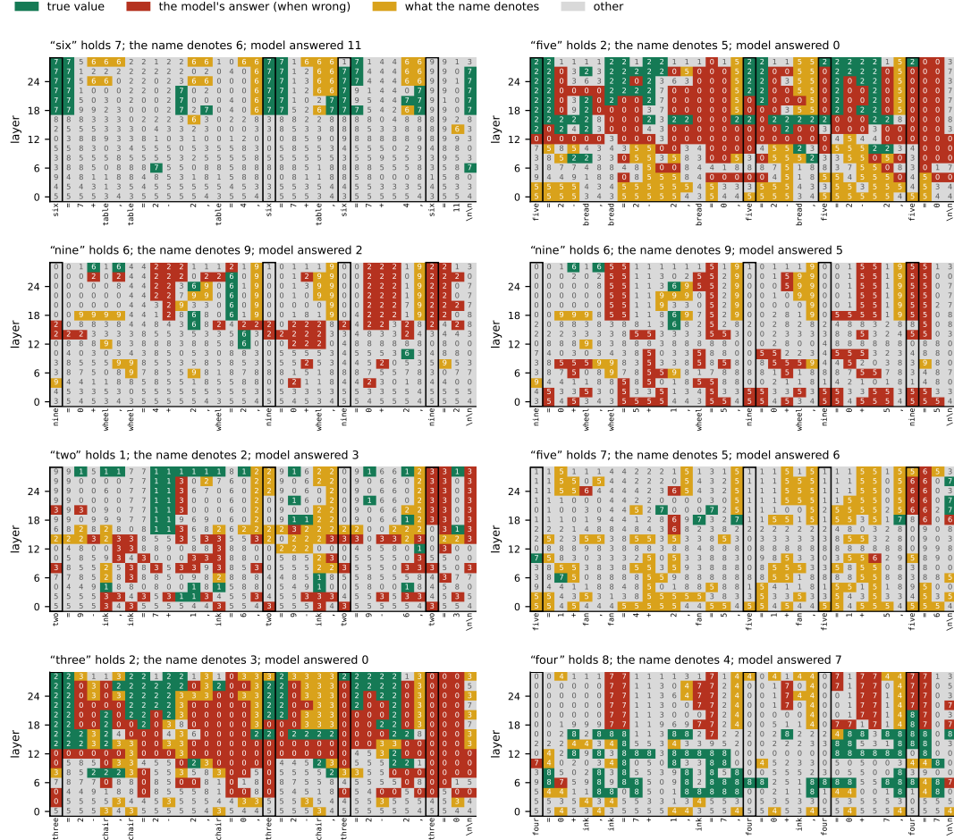
Figure 5: The probes of Figure 4 applied to the model’s own generated chain rather than to a force-decoded gold chain, for the eight level-3 incongruent problems that Llama-3.2-3B answered wrongly under CoT (the first 8 of 108 wrong answers in 2,000 instances). Probes are trained on neutral problems at the step that writes the variable’s value and applied at every generated token and every second layer; colours as in Figure 4, boxed columns the name’s own tokens. With eight instances this is a picture, not a rate: the states hold the value the model is about to write (red) in the late layers, and the name’s value (amber) is confined to the early layers at and after the name’s tokens.
