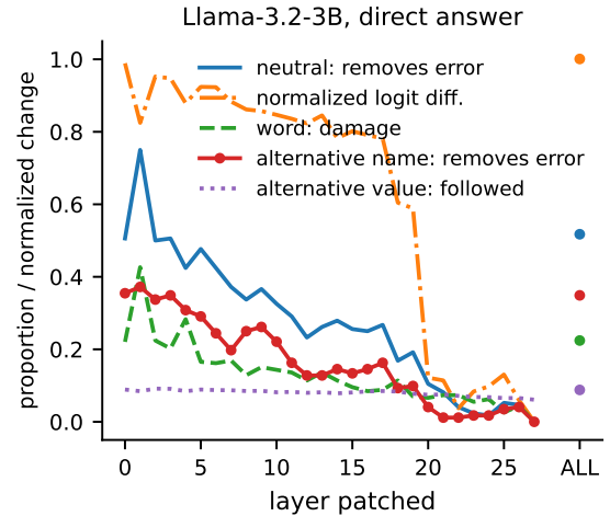
Figure 2: Llama-3.2-3B, answer-only: queried-variable name errors removed by layer, with neutral-word damage and alternative-name controls.
