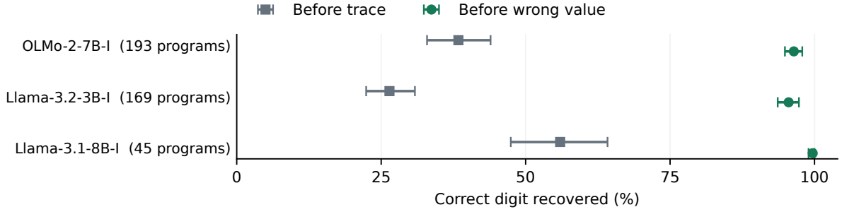
Figure 2: Correct-digit recovery on name-suggested wrong writes; counts are unique programs (95% intervals). I: instruction-tuned.
