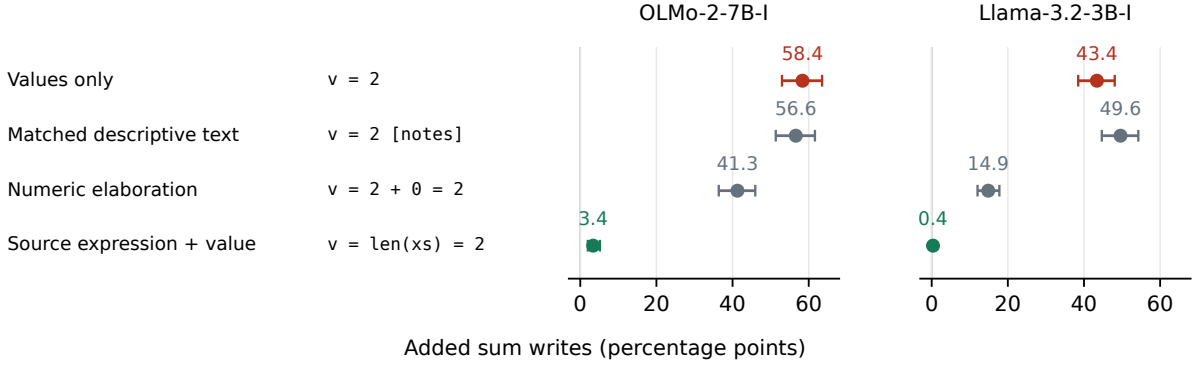
Figure 3: Demonstration-format controls (95% intervals). [notes]: matched descriptive text. I: instruction-tuned.
