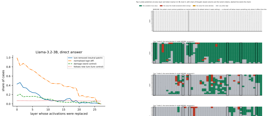
Figure 3: Lure errors removed by patching the name’s tokens from the neutral twin, by layer, direct regime, with the neutral-word control patch (damage) and the alternative-lure patch.
