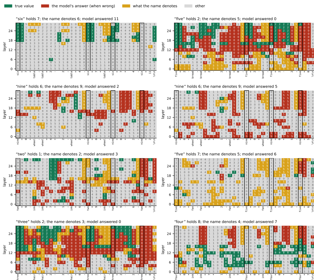
Figure 28: The own-chain probe figure at full size.
