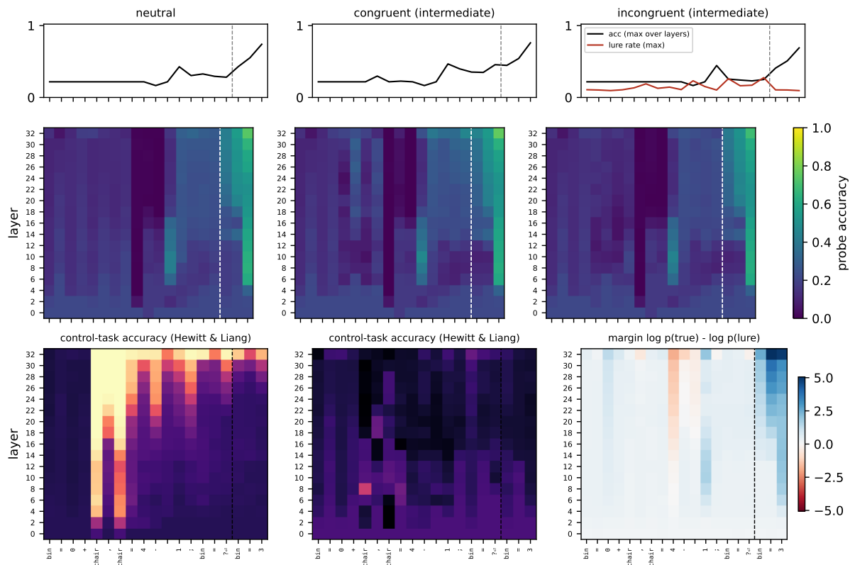
Figure 32: Llama-3.1-8B, direct regime, intermediate variable.
