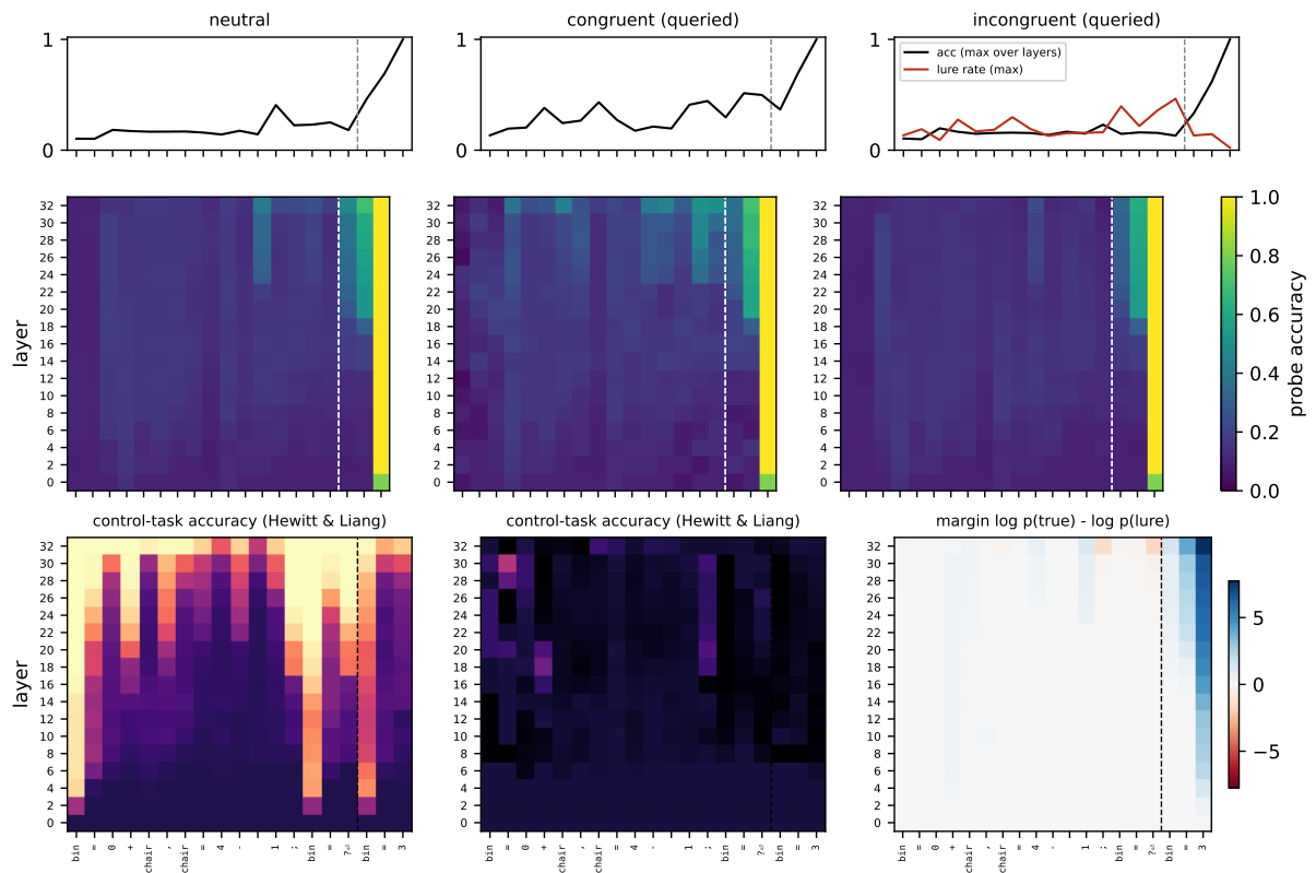
Figure 35: Llama-3.1-8B, direct regime, queried variable.
