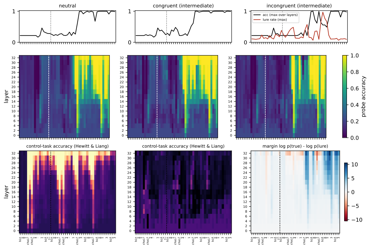
Figure 31: Llama-3.1-8B, chain-of-thought regime, intermediate variable.
