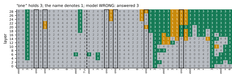
Figure 17: A second problem, intermediate variable.
