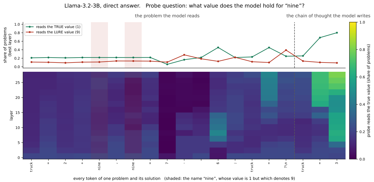
Figure 9: Per-token probes, direct regime, intermediate variable.
