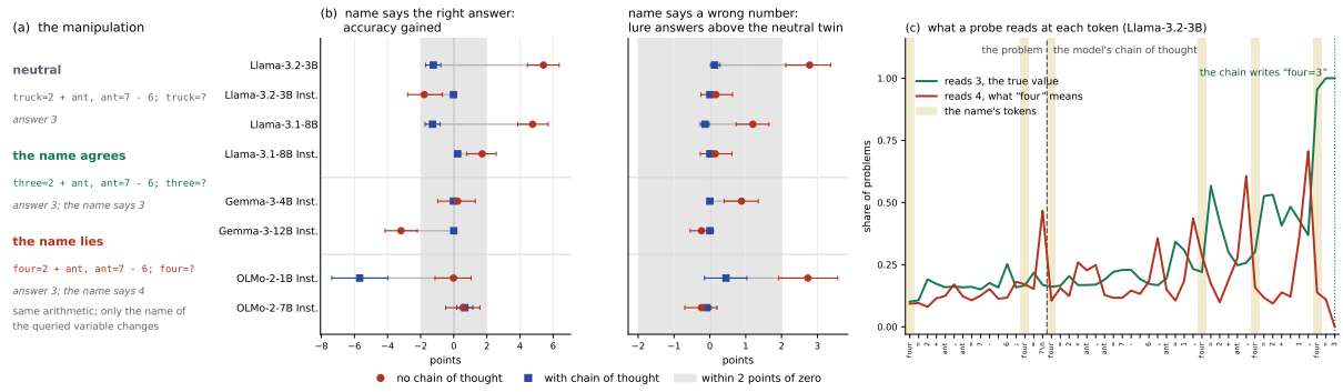
Figure 6: Figure 1 at full size.
