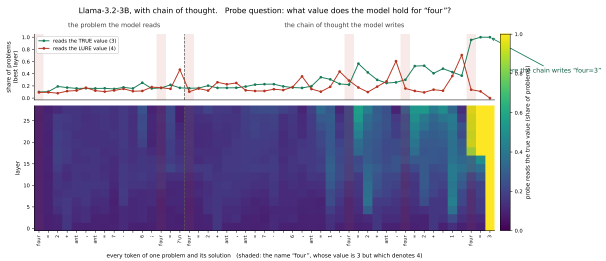
Figure 8: Per-token probes, chain-of-thought regime, queried variable.
