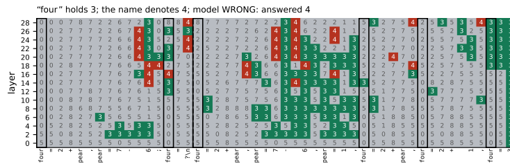
Figure 12: A second problem answered with the lure.
