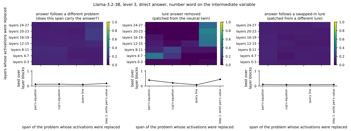
Figure 21: The same grids in the direct regime.
