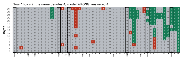
Figure 13: A third problem answered with the lure.
