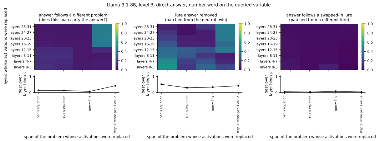
Figure 37: Llama-3.1-8B, patching grids, direct regime, queried variable.
