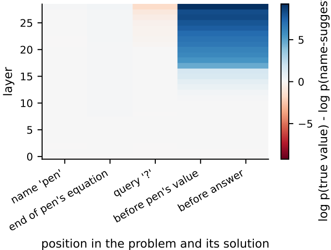
with chain of thought
