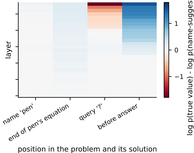
direct answer
