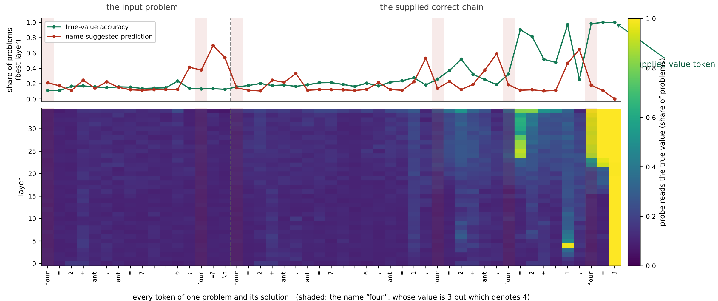
Gemma-3-4B-it, with chain of thought: queried-value probe readouts
