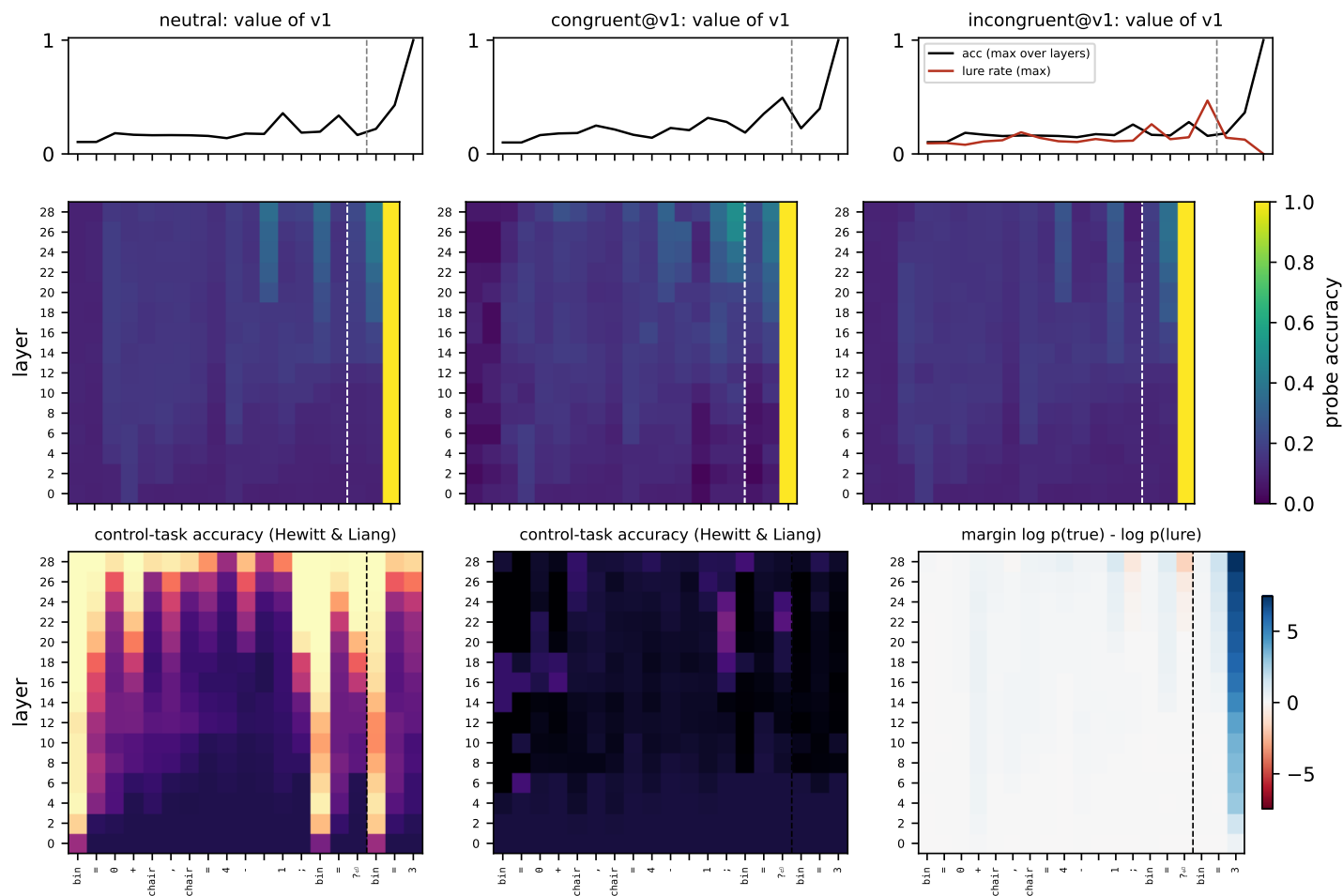
Figure 26: kudo_fig2_llama32-3b_L3_direct_v1.
