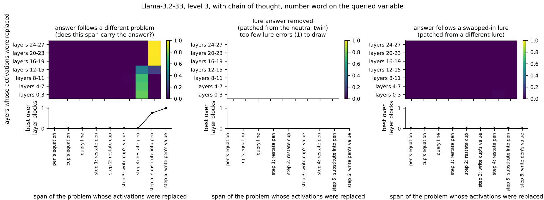
Figure 27: kudo_fig5_llama32-3b_L3_cot_v1.
