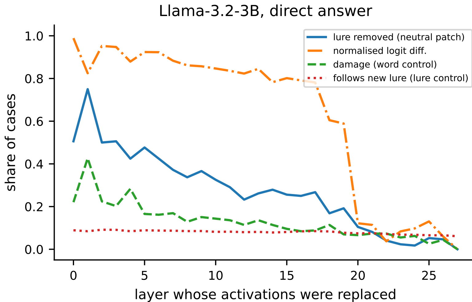
Figure 24: fig3_patching_llama32-3b_L3_v1.
