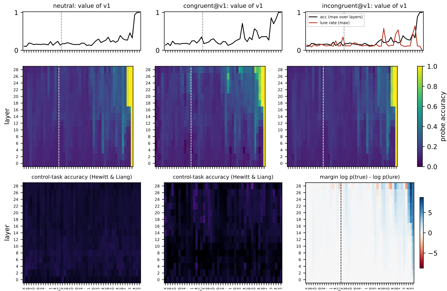
Figure 25: kudo_fig2_llama32-3b_L3_cot_v1.
