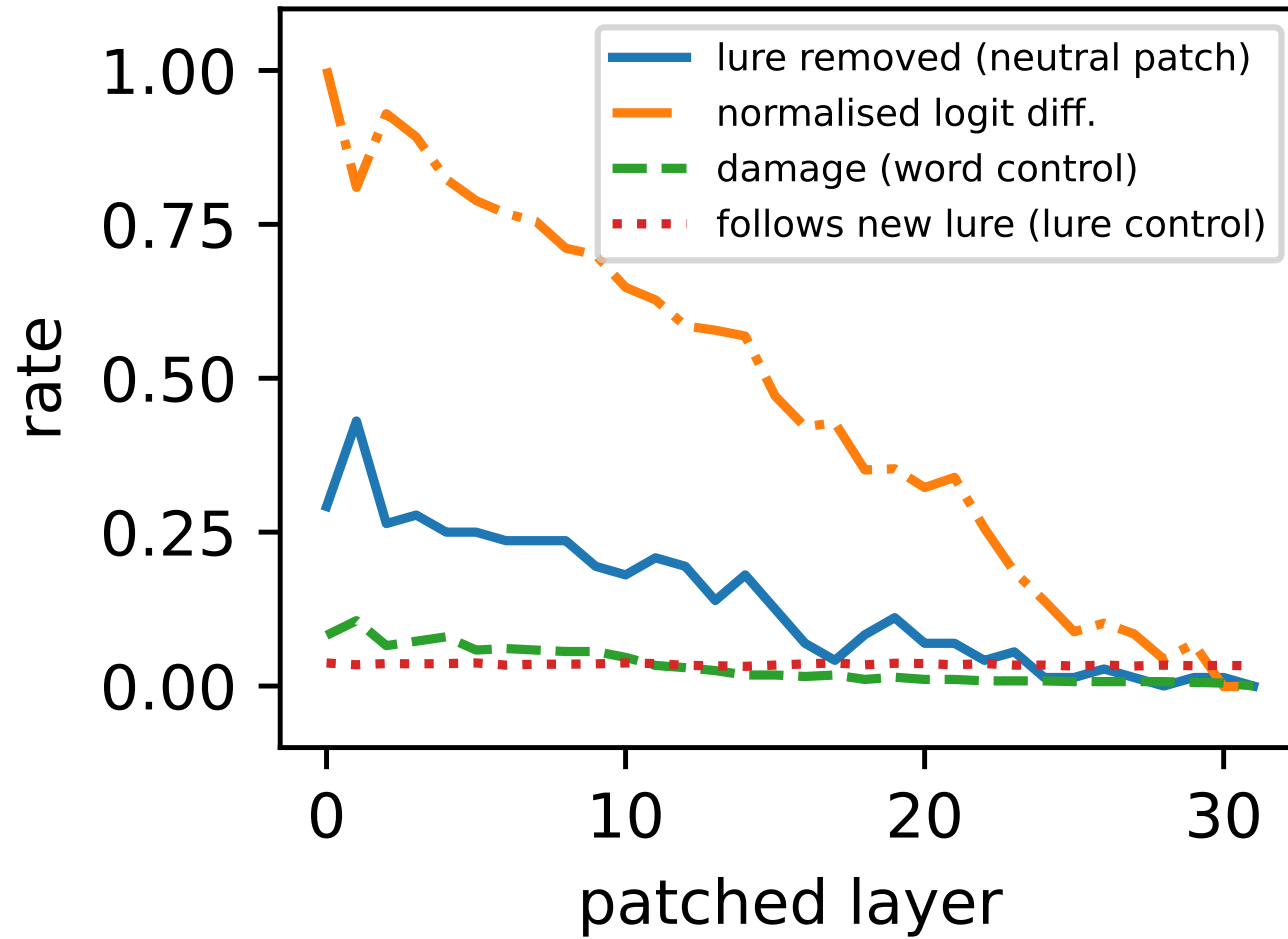
Figure 23: fig3_patching_llama31-8b_L3_v2.
