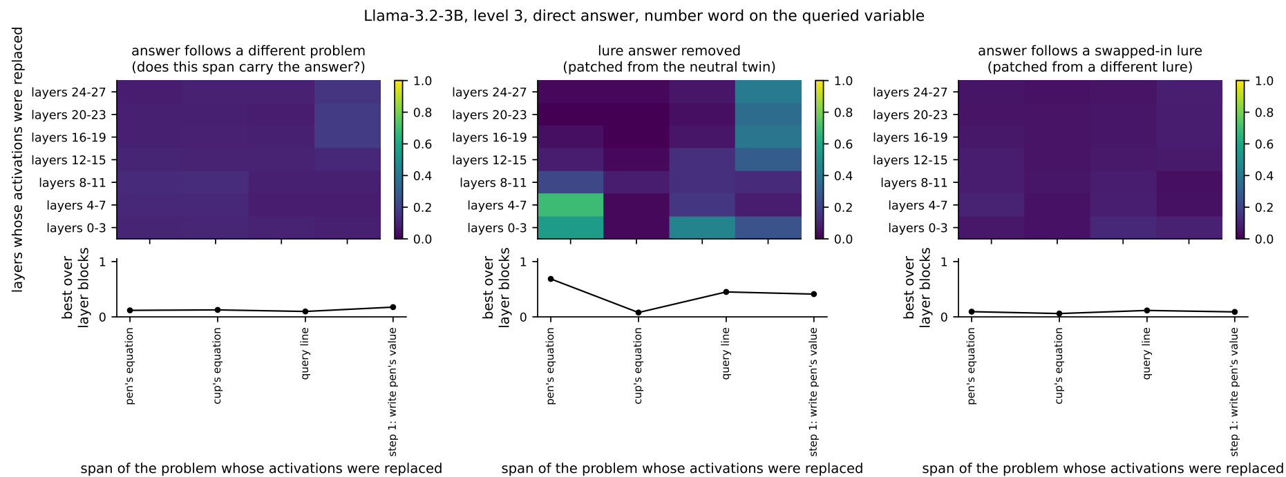
Figure 28: kudo_fig5_llama32-3b_L3_direct_v1.
