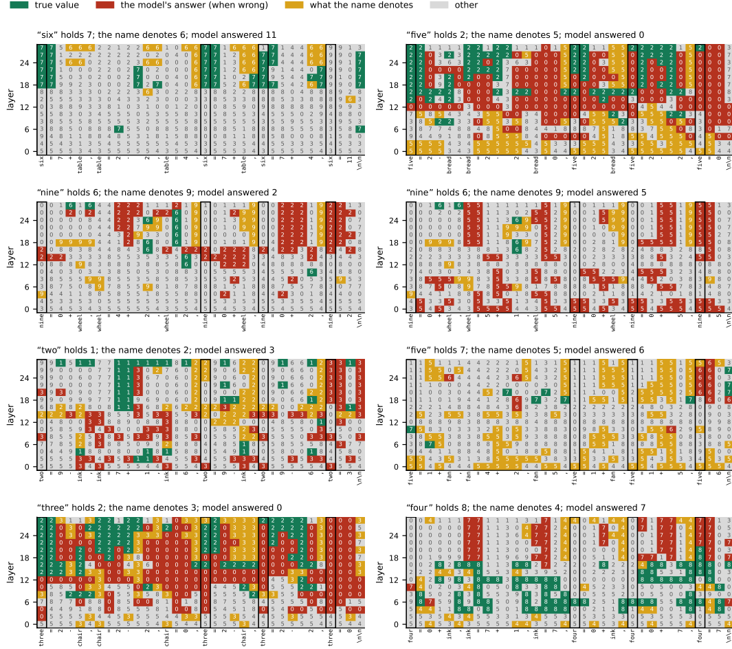
Figure 5: The probes of Figure 4 applied to the model’s own generated chain rather than to a force-decoded gold chain, for the eight level-3 incongruent problems that Llama-3.2-3B answered wrongly under CoT (the first 8 of 108 wrong answers in 2,000 instances). Probes are trained on neutral problems at the step that writes the variable’s value and applied at every generated token and every second layer; colours as in Figure 4, boxed columns the name’s own tokens. With eight instances this is a picture, not a rate: the states hold the value the model is about to write (red) in the late layers, and the name’s value (amber) is confined to the early layers at and after the name’s tokens.
