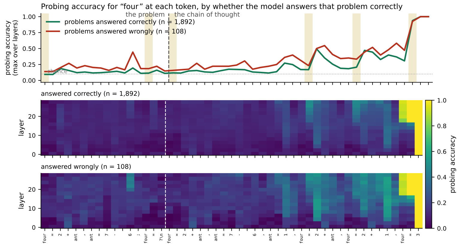
Figure 10: Probing accuracy split by whether the model answers the problem correctly on its own, with the layer sweep for each half.
