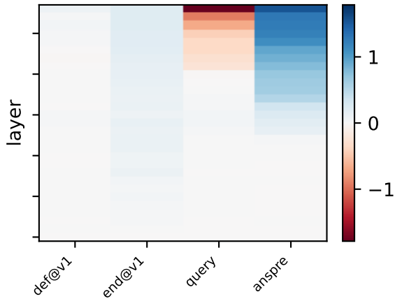
llama32-3b direct: \log p(\text{true}) - \log p(\text{lure})
